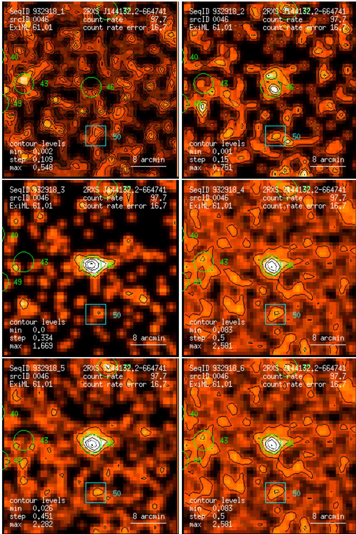
Figure 46: RASS 932918: detection 0046: band rate images, Gaussian filter: (1) PSPC channels 11 – 41, (2) 52 – 90, (3) 91 – 201, (4) 11 – 235, (5) 52 – 201, (6) 11 – 201. Broad band rates in counts/ks. Band rate contour levels in counts/ks/arcmin 2 .
