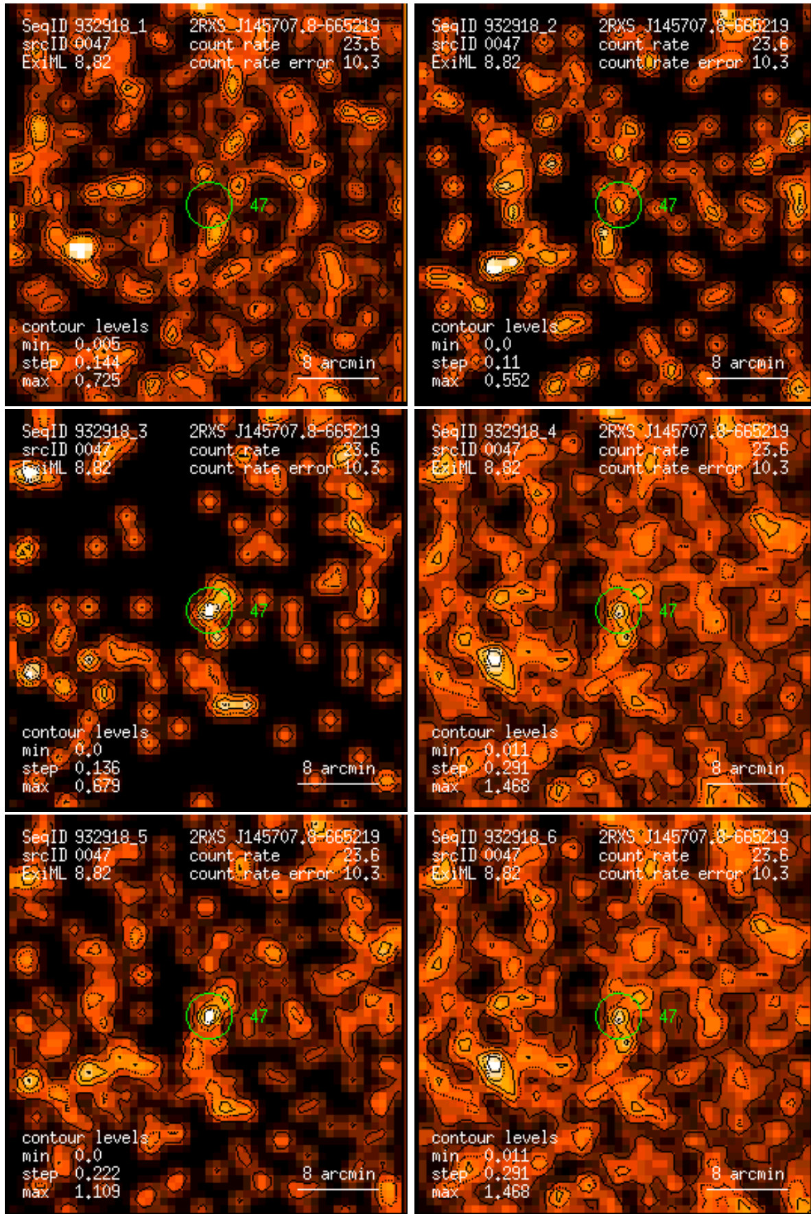
Figure 47: RASS 932918: detection 0047: band rate images, Gaussian filter: (1) PSPC channels 11 – 41, (2) 52 – 90, (3) 91 – 201, (4) 11 – 235, (5) 52 – 201, (6) 11 – 201. Broad band rates in counts/ks. Band rate contour levels in counts/ks/arcmin 2 .
