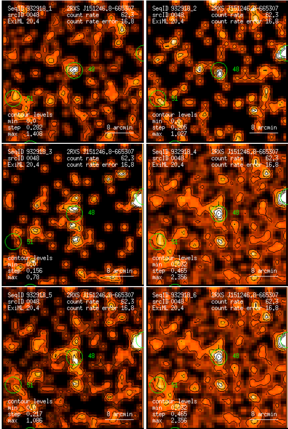
Figure 48: RASS 932918: detection 0048: band rate images, Gaussian filter: (1) PSPC channels 11 – 41, (2) 52 – 90, (3) 91 – 201, (4) 11 – 235, (5) 52 – 201, (6) 11 – 201. Broad band rates in counts/ks. Band rate contour levels in counts/ks/arcmin 2 .
