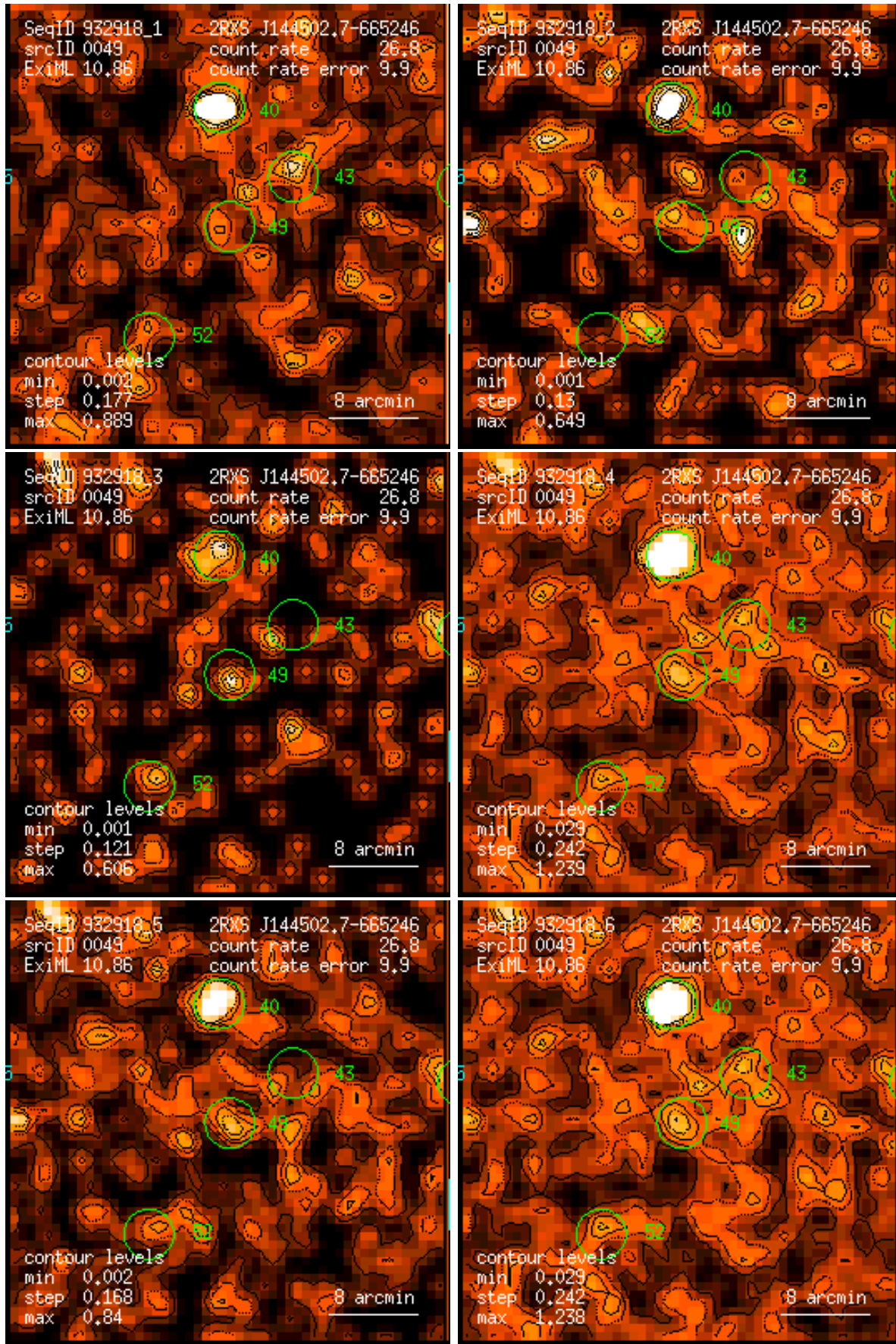
Figure 49: RASS 932918: detection 0049: band rate images, Gaussian filter: (1) PSPC channels 11 – 41, (2) 52 – 90, (3) 91 – 201, (4) 11 – 235, (5) 52 – 201, (6) 11 – 201. Broad band rates in counts/ks. Band rate contour levels in counts/ks/arcmin 2 .
