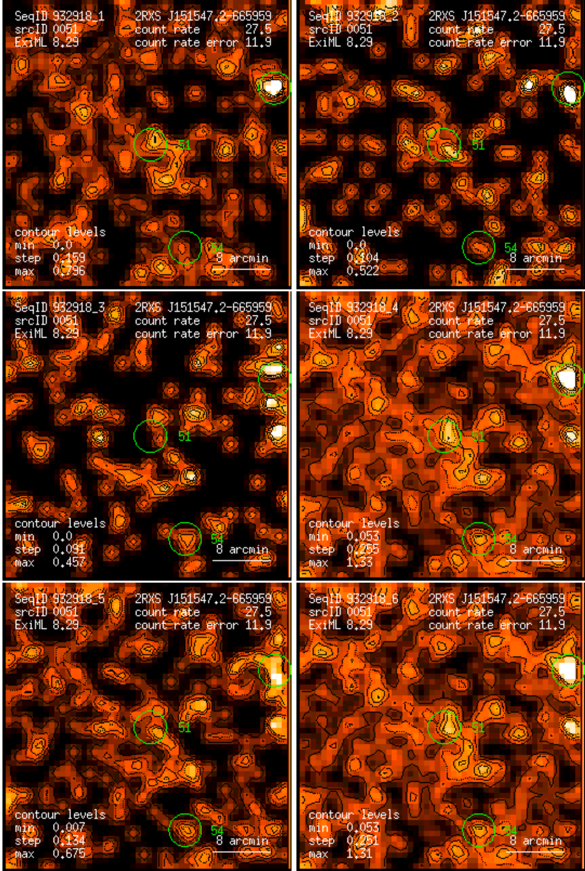
Figure 51: RASS 932918: detection 0051: band rate images, Gaussian filter: (1) PSPC channels 11 – 41, (2) 52 – 90, (3) 91 – 201, (4) 11 – 235, (5) 52 – 201, (6) 11 – 201. Broad band rates in counts/ks. Band rate contour levels in counts/ks/arcmin 2 .
