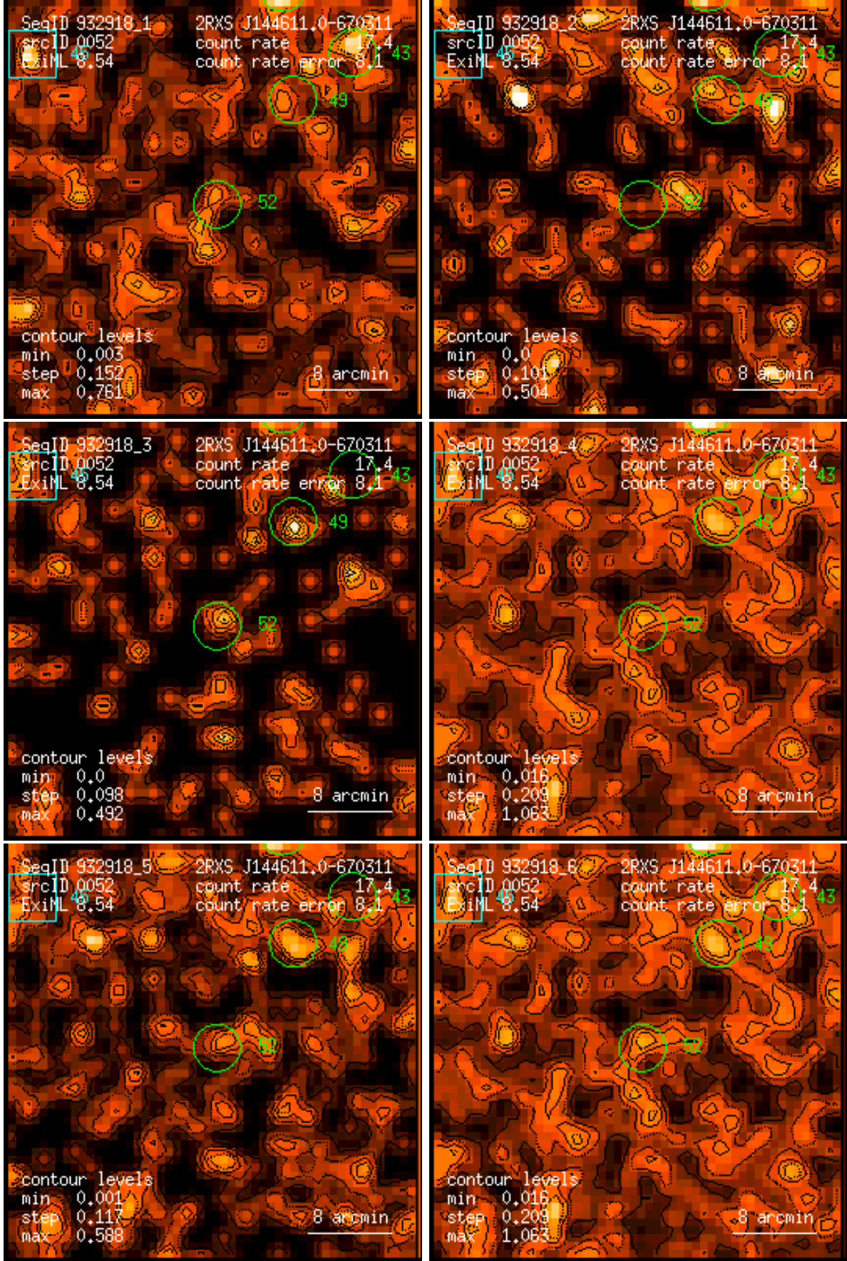
Figure 52: RASS 932918: detection 0052: band rate images, Gaussian filter: (1) PSPC channels 11 – 41, (2) 52 – 90, (3) 91 – 201, (4) 11 – 235, (5) 52 – 201, (6) 11 – 201. Broad band rates in counts/ks. Band rate contour levels in counts/ks/arcmin 2 .
