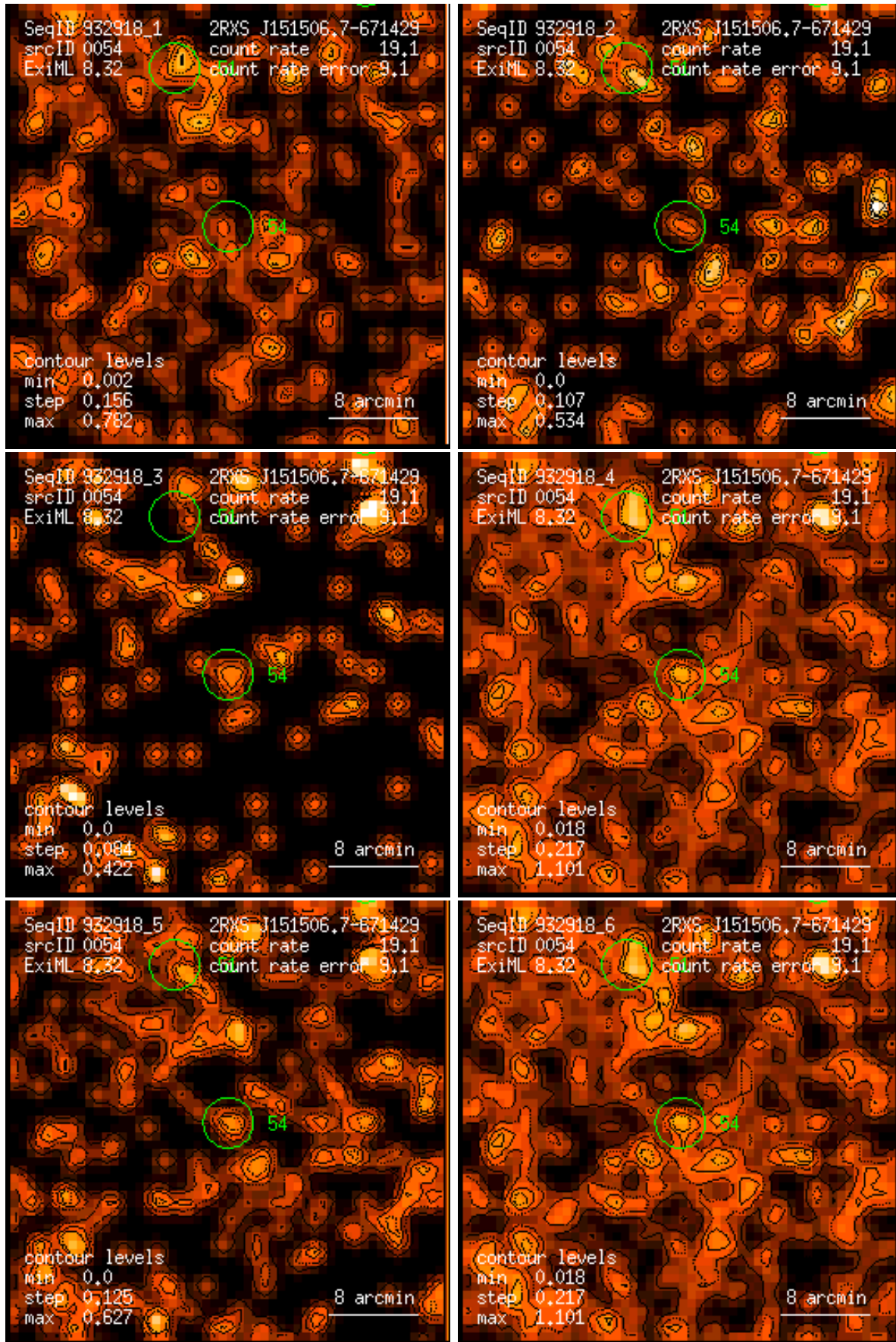
Figure 54: RASS 932918: detection 0054: band rate images, Gaussian filter: (1) PSPC channels 11 – 41, (2) 52 – 90, (3) 91 – 201, (4) 11 – 235, (5) 52 – 201, (6) 11 – 201. Broad band rates in counts/ks. Band rate contour levels in counts/ks/arcmin 2 .
