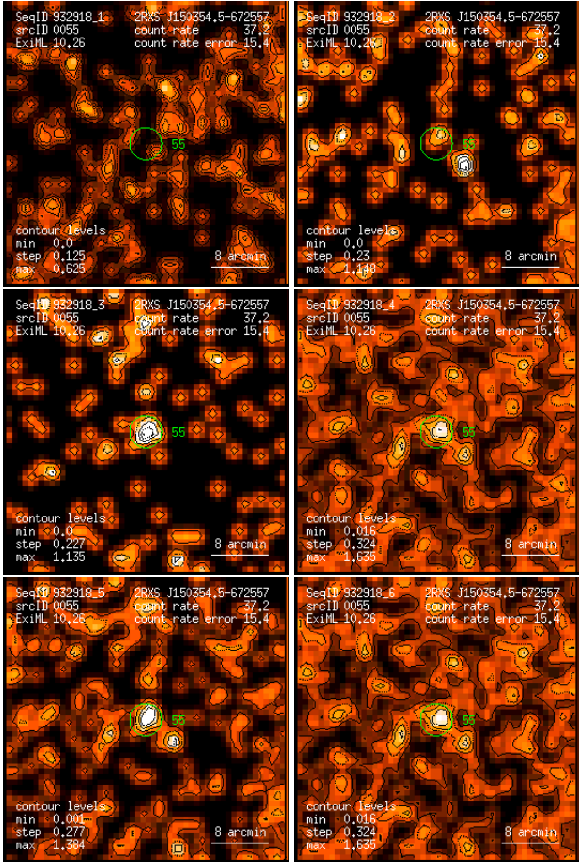
Figure 55: RASS 932918: detection 0055: band rate images, Gaussian filter: (1) PSPC channels 11 – 41, (2) 52 – 90, (3) 91 – 201, (4) 11 – 235, (5) 52 – 201, (6) 11 – 201. Broad band rates in counts/ks. Band rate contour levels in counts/ks/arcmin 2 .
