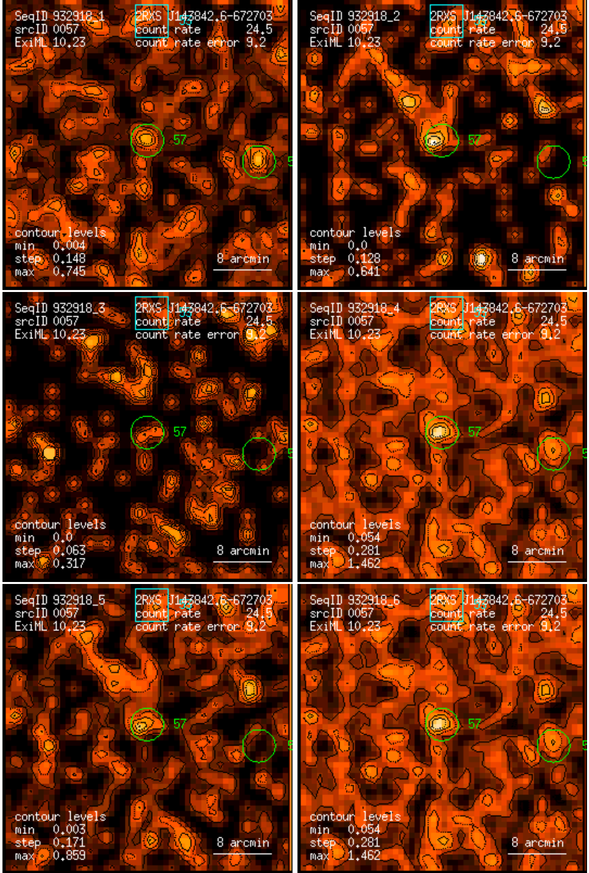
Figure 57: RASS 932918: detection 0057: band rate images, Gaussian filter: (1) PSPC channels 11 – 41, (2) 52 – 90, (3) 91 – 201, (4) 11 – 235, (5) 52 – 201, (6) 11 – 201. Broad band rates in counts/ks. Band rate contour levels in counts/ks/arcmin 2 .
