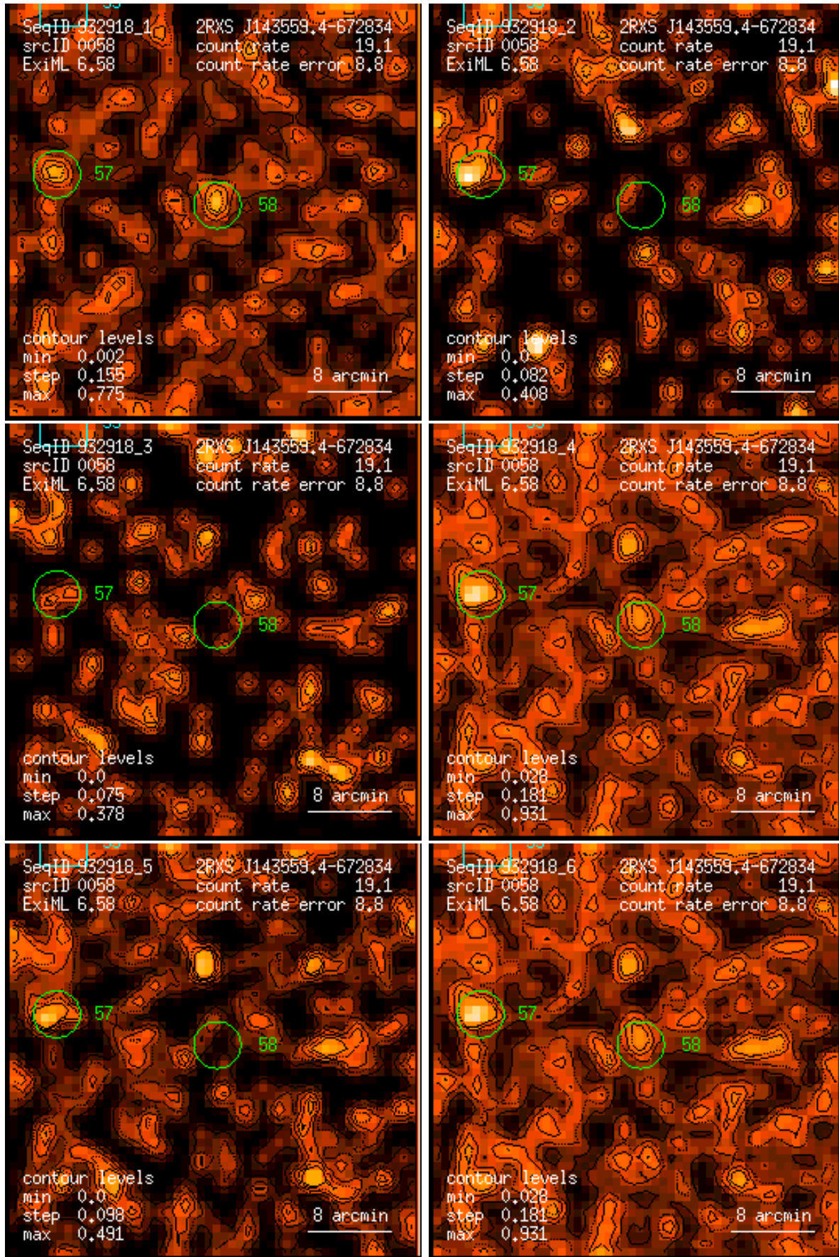
Figure 58: RASS 932918: detection 0058: band rate images, Gaussian filter: (1) PSPC channels 11 – 41, (2) 52 – 90, (3) 91 – 201, (4) 11 – 235, (5) 52 – 201, (6) 11 – 201. Broad band rates in counts/ks. Band rate contour levels in counts/ks/arcmin 2 .
