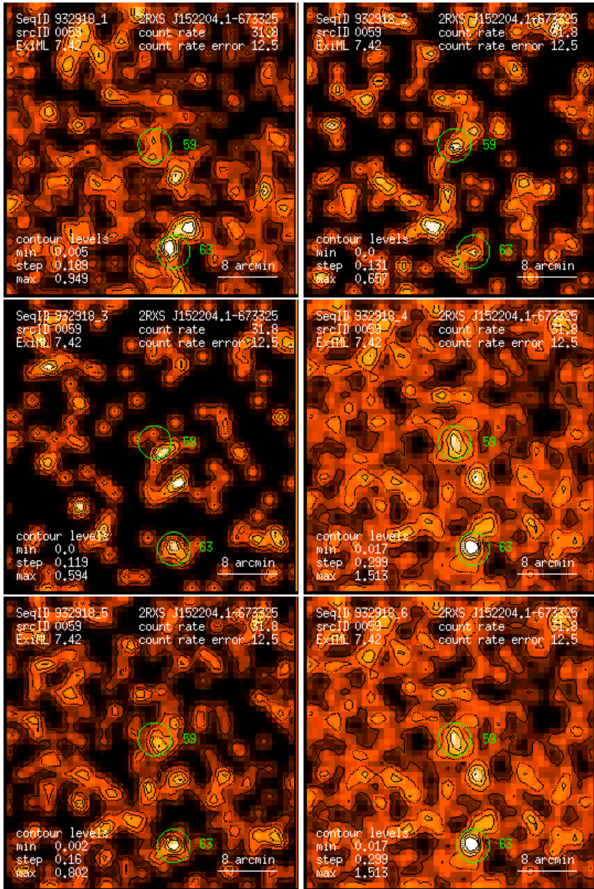
Figure 59: RASS 932918: detection 0059: band rate images, Gaussian filter: (1) PSPC channels 11 – 41, (2) 52 – 90, (3) 91 – 201, (4) 11 – 235, (5) 52 – 201, (6) 11 – 201. Broad band rates in counts/ks. Band rate contour levels in counts/ks/arcmin 2 .
