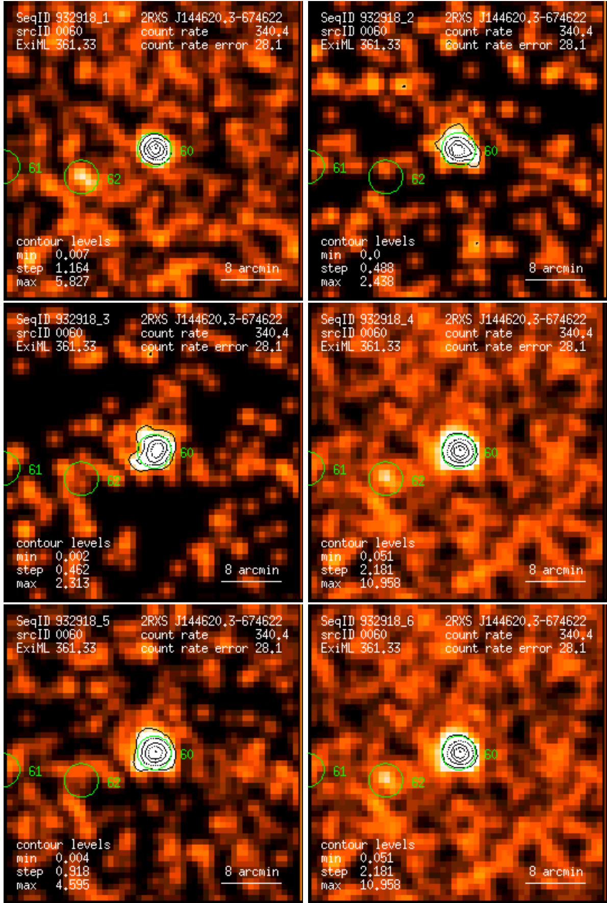
Figure 60: RASS 932918: detection 0060: band rate images, Gaussian filter: (1) PSPC channels 11 – 41, (2) 52 – 90, (3) 91 – 201, (4) 11 – 235, (5) 52 – 201, (6) 11 – 201. Broad band rates in counts/ks. Band rate contour levels in counts/ks/arcmin 2 .
