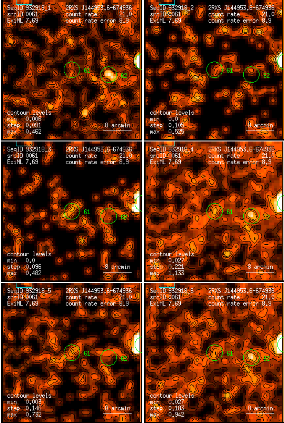
Figure 61: RASS 932918: detection 0061: band rate images, Gaussian filter: (1) PSPC channels 11 – 41, (2) 52 – 90, (3) 91 – 201, (4) 11 – 235, (5) 52 – 201, (6) 11 – 201. Broad band rates in counts/ks. Band rate contour levels in counts/ks/arcmin 2 .
