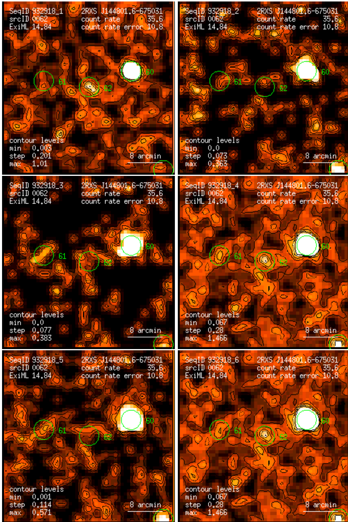
Figure 62: RASS 932918: detection 0062: band rate images, Gaussian filter: (1) PSPC channels 11 – 41, (2) 52 – 90, (3) 91 – 201, (4) 11 – 235, (5) 52 – 201, (6) 11 – 201. Broad band rates in counts/ks. Band rate contour levels in counts/ks/arcmin 2 .
