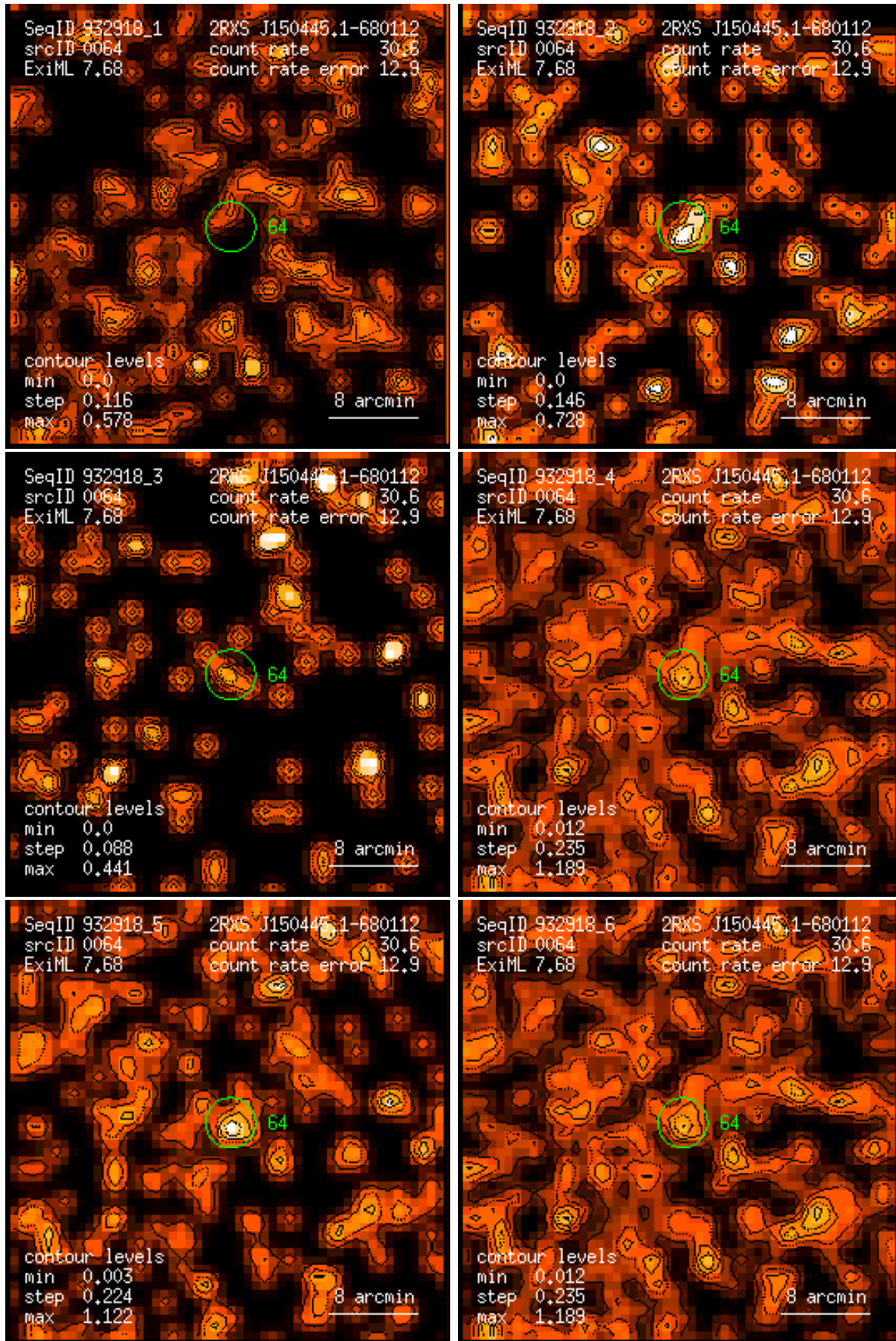
Figure 64: RASS 932918: detection 0064: band rate images, Gaussian filter: (1) PSPC channels 11 – 41, (2) 52 – 90, (3) 91 – 201, (4) 11 – 235, (5) 52 – 201, (6) 11 – 201. Broad band rates in counts/ks. Band rate contour levels in counts/ks/arcmin 2 .
