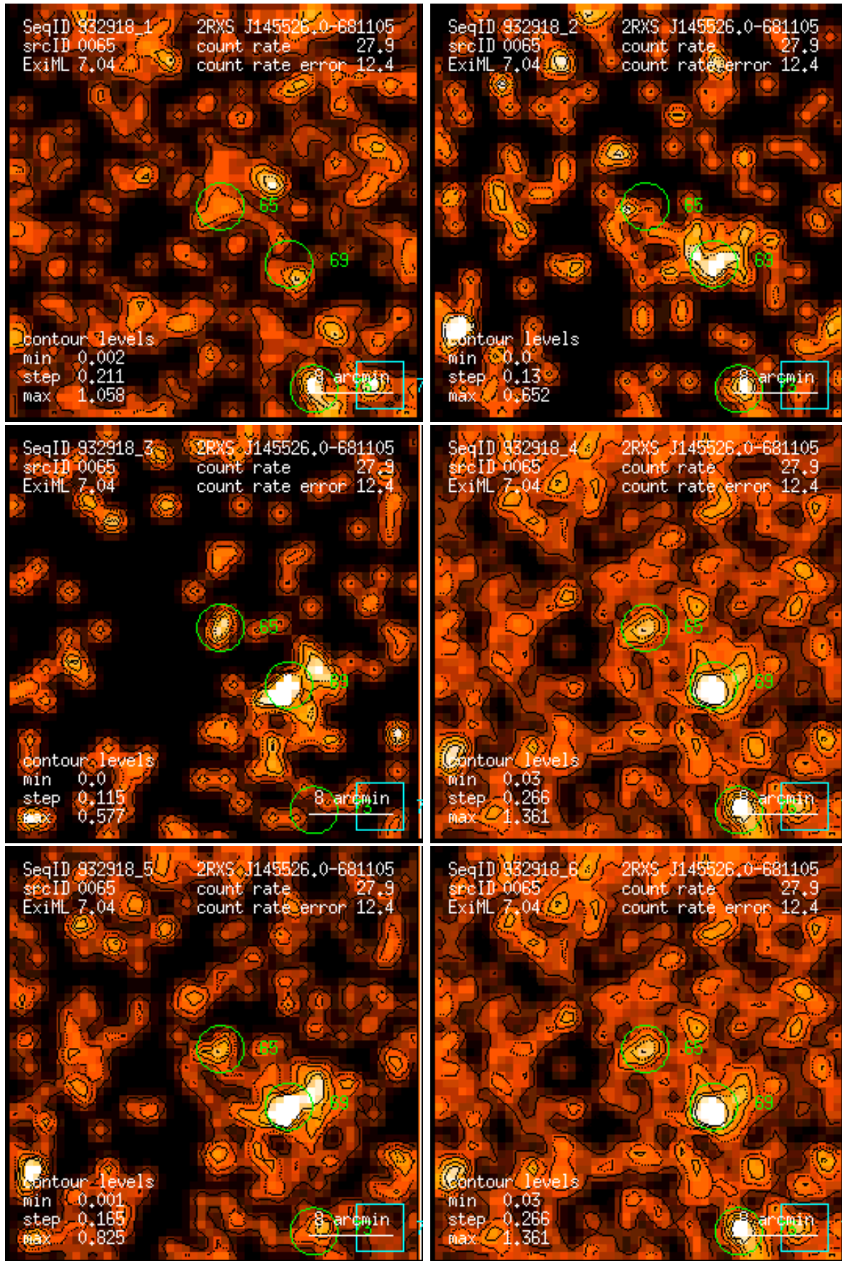
Figure 65: RASS 932918: detection 0065: band rate images, Gaussian filter: (1) PSPC channels 11 – 41, (2) 52 – 90, (3) 91 – 201, (4) 11 – 235, (5) 52 – 201, (6) 11 – 201. Broad band rates in counts/ks. Band rate contour levels in counts/ks/arcmin 2 .
