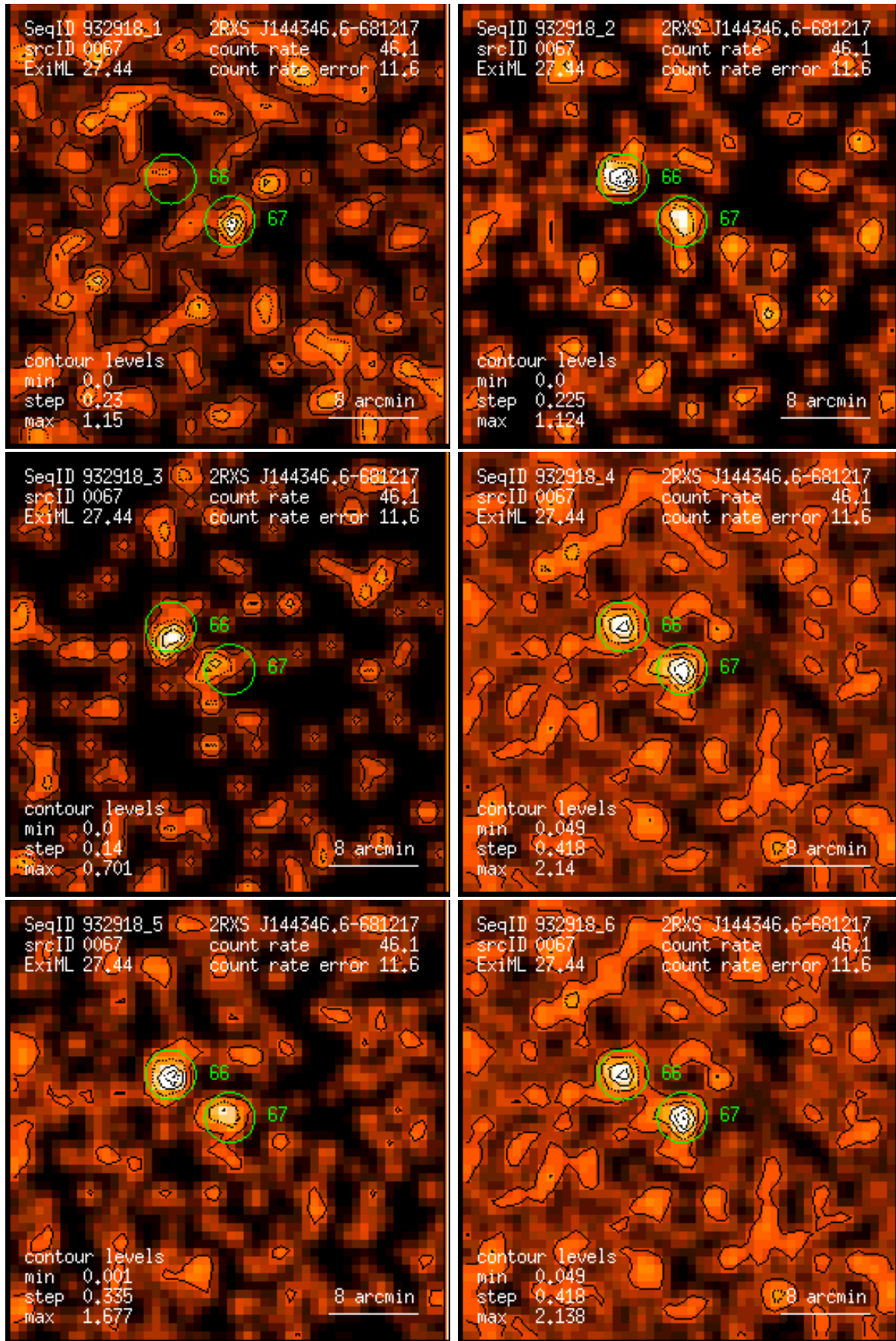
Figure 67: RASS 932918: detection 0067: band rate images, Gaussian filter: (1) PSPC channels 11 – 41, (2) 52 – 90, (3) 91 – 201, (4) 11 – 235, (5) 52 – 201, (6) 11 – 201. Broad band rates in counts/ks. Band rate contour levels in counts/ks/arcmin 2 .
