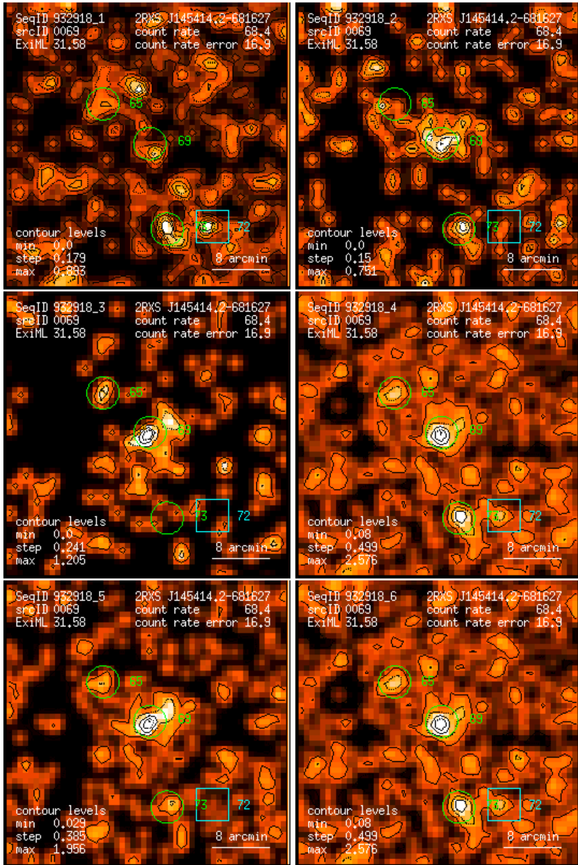
Figure 69: RASS 932918: detection 0069: band rate images, Gaussian filter: (1) PSPC channels 11 – 41, (2) 52 – 90, (3) 91 – 201, (4) 11 – 235, (5) 52 – 201, (6) 11 – 201. Broad band rates in counts/ks. Band rate contour levels in counts/ks/arcmin 2 .
