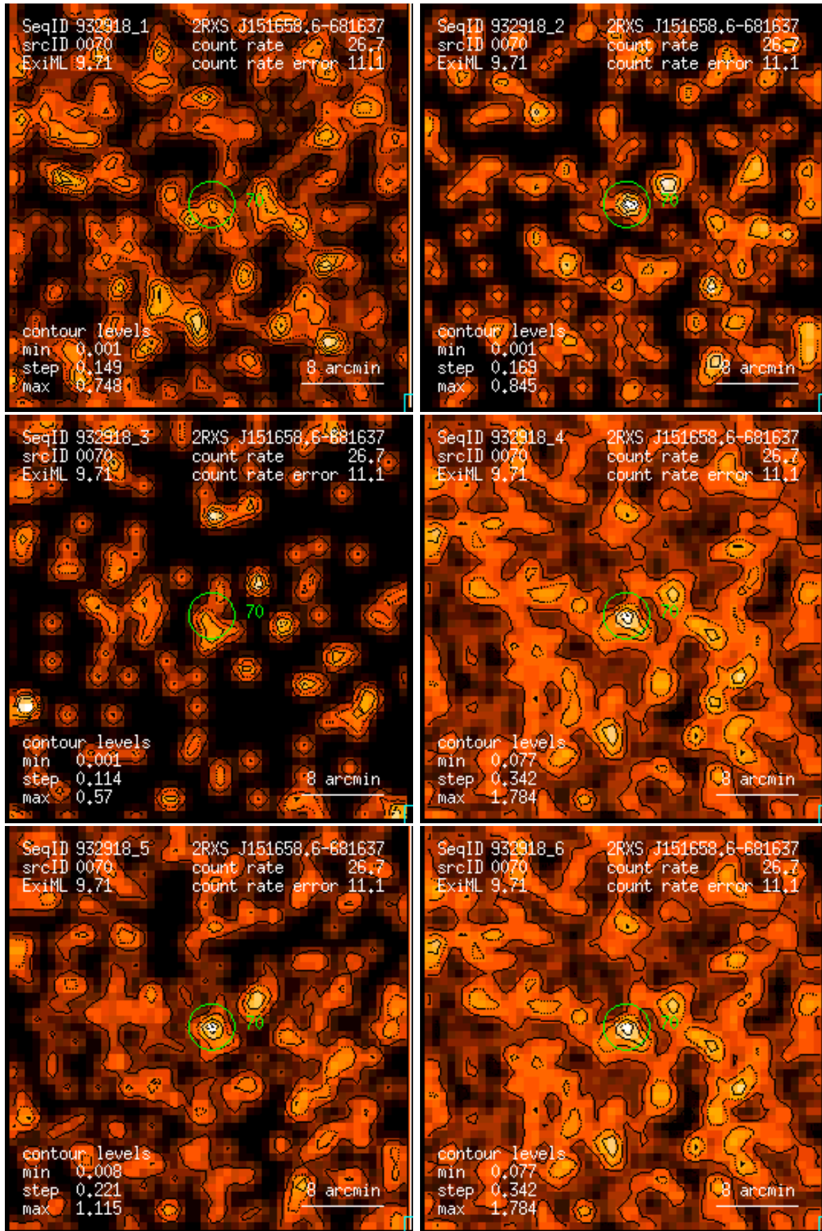
Figure 70: RASS 932918: detection 0070: band rate images, Gaussian filter: (1) PSPC channels 11 – 41, (2) 52 – 90, (3) 91 – 201, (4) 11 – 235, (5) 52 – 201, (6) 11 – 201. Broad band rates in counts/ks. Band rate contour levels in counts/ks/arcmin 2 .
