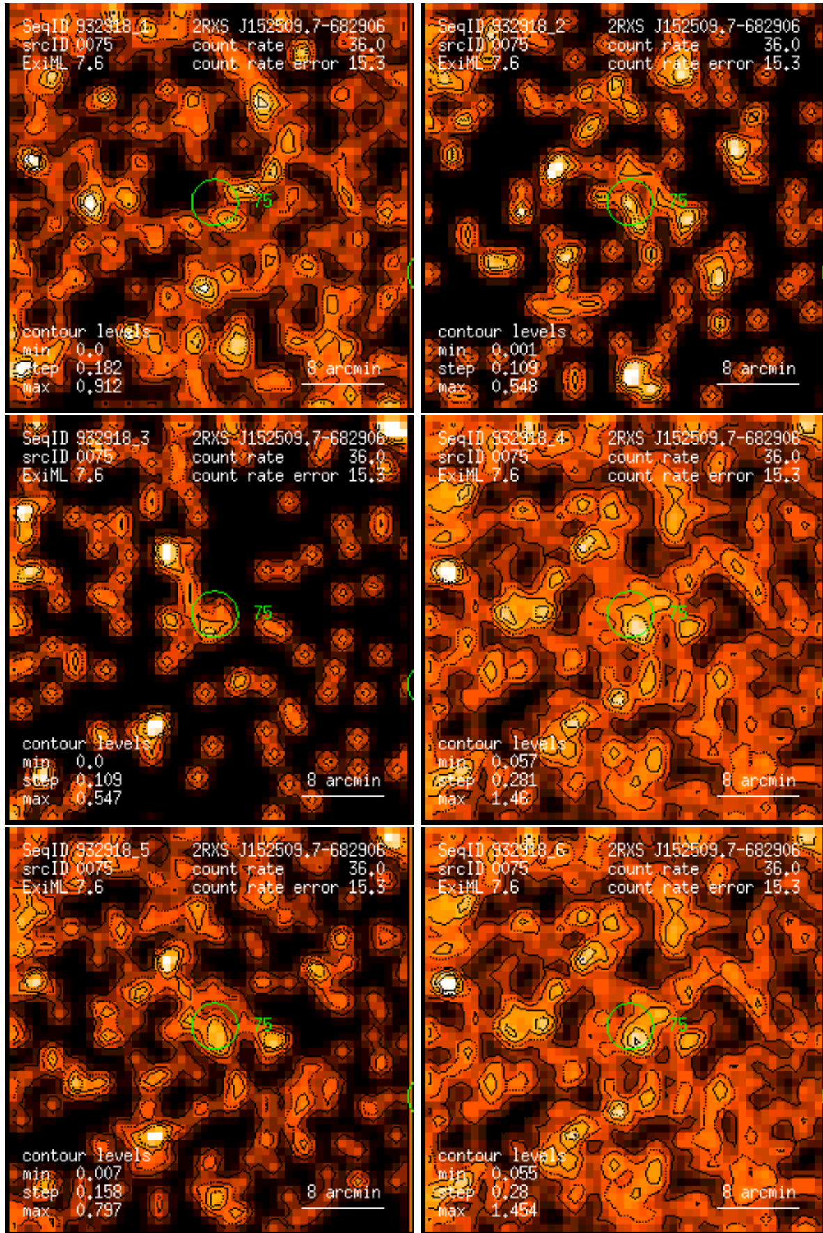
Figure 75: RASS 932918: detection 0075: band rate images, Gaussian filter: (1) PSPC channels 11 – 41, (2) 52 – 90, (3) 91 – 201, (4) 11 – 235, (5) 52 – 201, (6) 11 – 201. Broad band rates in counts/ks. Band rate contour levels in counts/ks/arcmin 2 .
