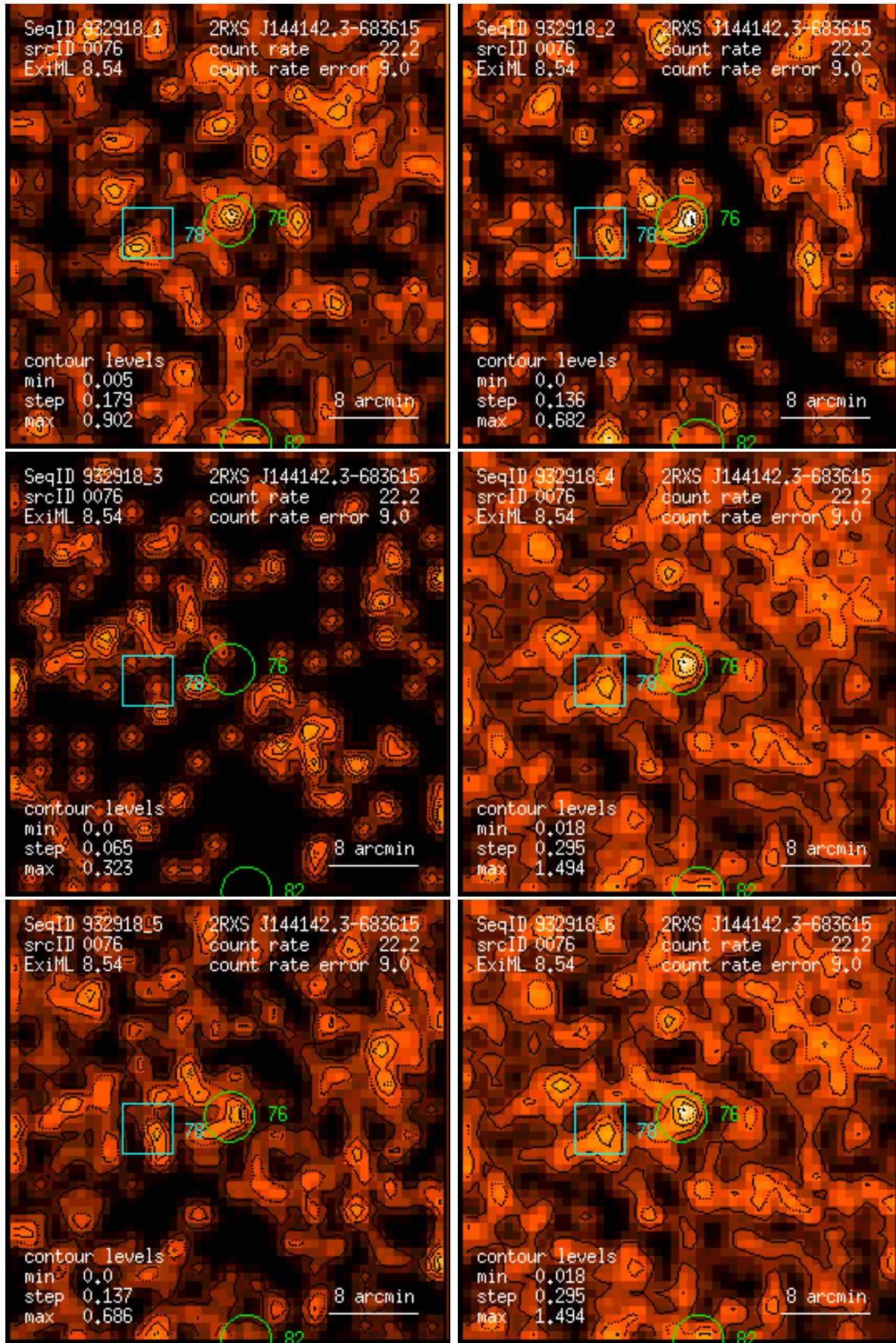
Figure 76: RASS 932918: detection 0076: band rate images, Gaussian filter: (1) PSPC channels 11 – 41, (2) 52 – 90, (3) 91 – 201, (4) 11 – 235, (5) 52 – 201, (6) 11 – 201. Broad band rates in counts/ks. Band rate contour levels in counts/ks/arcmin 2 .
