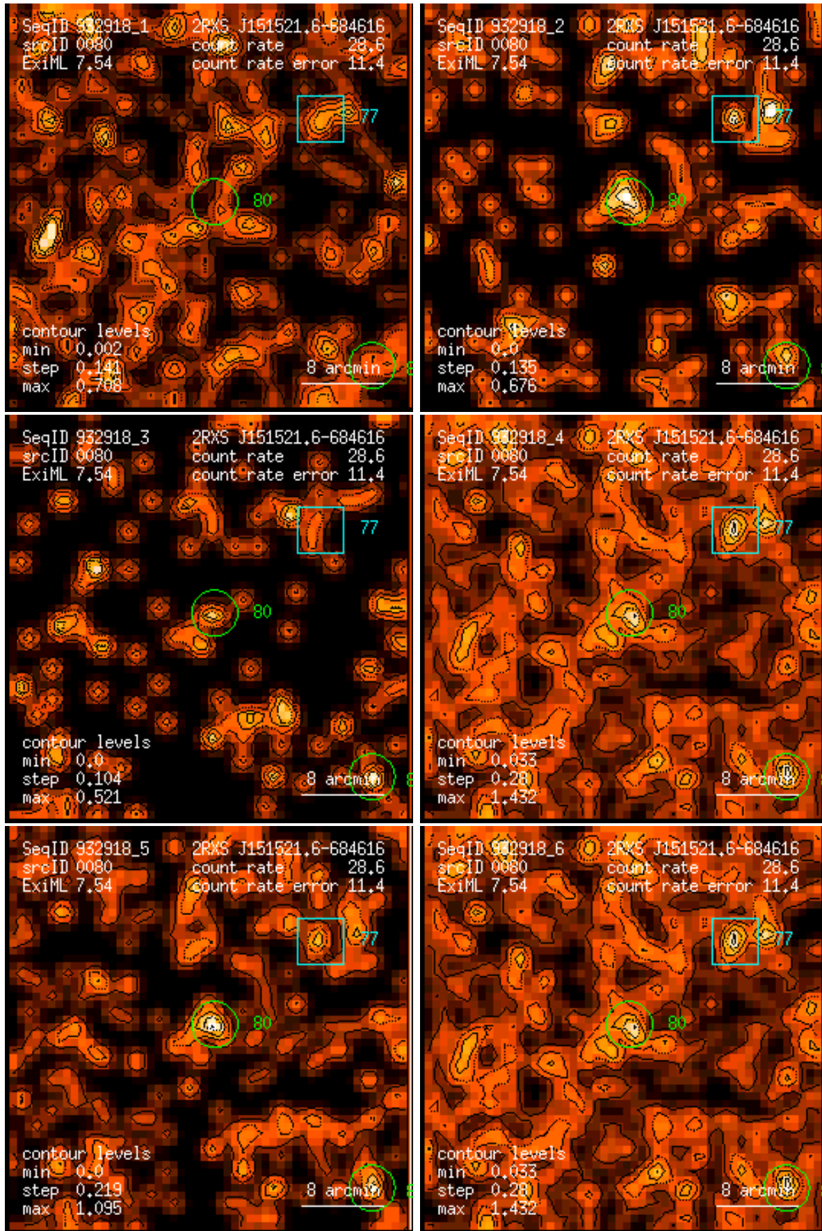
Figure 80: RASS 932918: detection 0080: band rate images, Gaussian filter: (1) PSPC channels 11 – 41, (2) 52 – 90, (3) 91 – 201, (4) 11 – 235, (5) 52 – 201, (6) 11 – 201. Broad band rates in counts/ks. Band rate contour levels in counts/ks/arcmin 2 .
