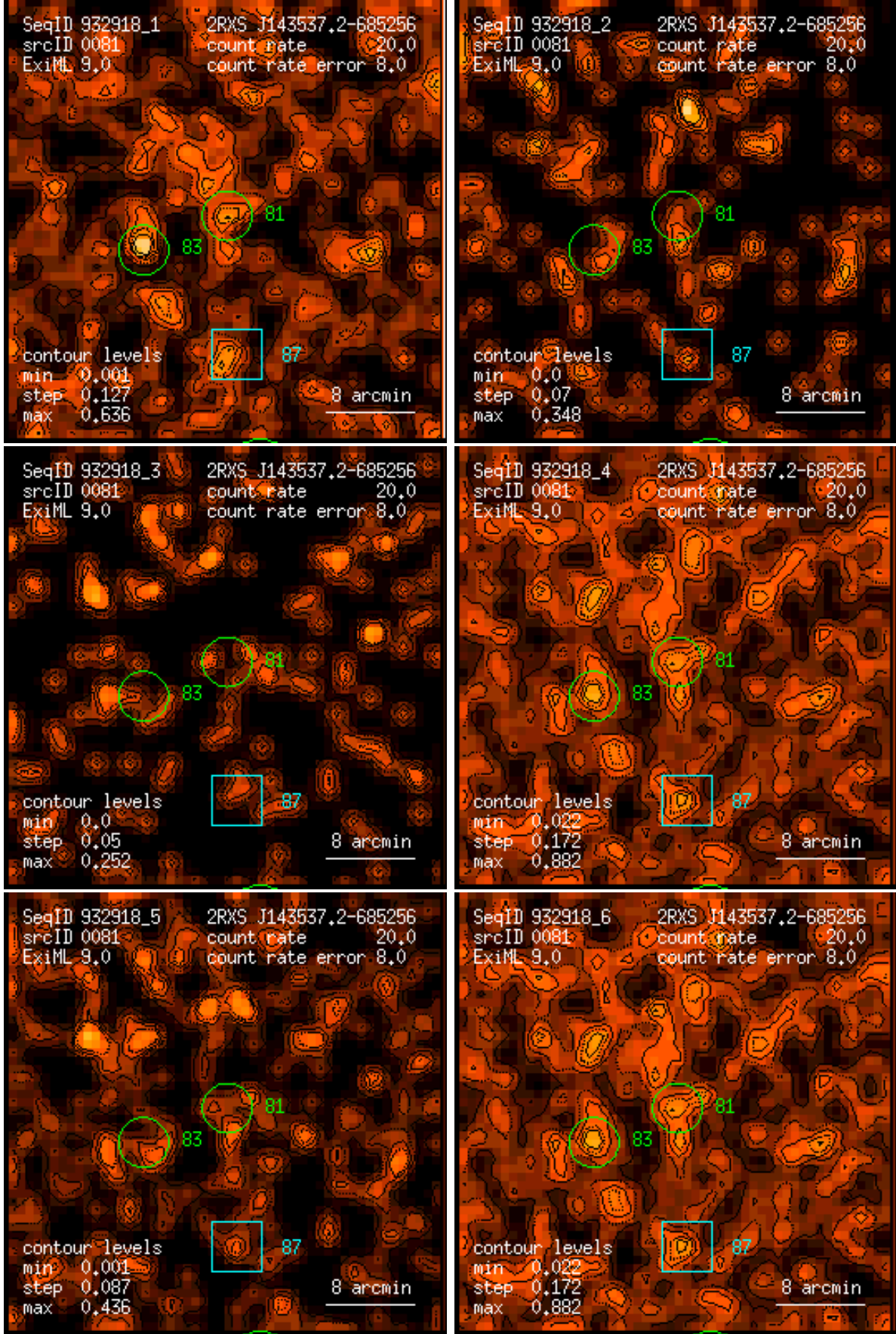
Figure 81: RASS 932918: detection 0081: band rate images, Gaussian filter: (1) PSPC channels 11 – 41, (2) 52 – 90, (3) 91 – 201, (4) 11 – 235, (5) 52 – 201, (6) 11 – 201. Broad band rates in counts/ks. Band rate contour levels in counts/ks/arcmin 2 .
