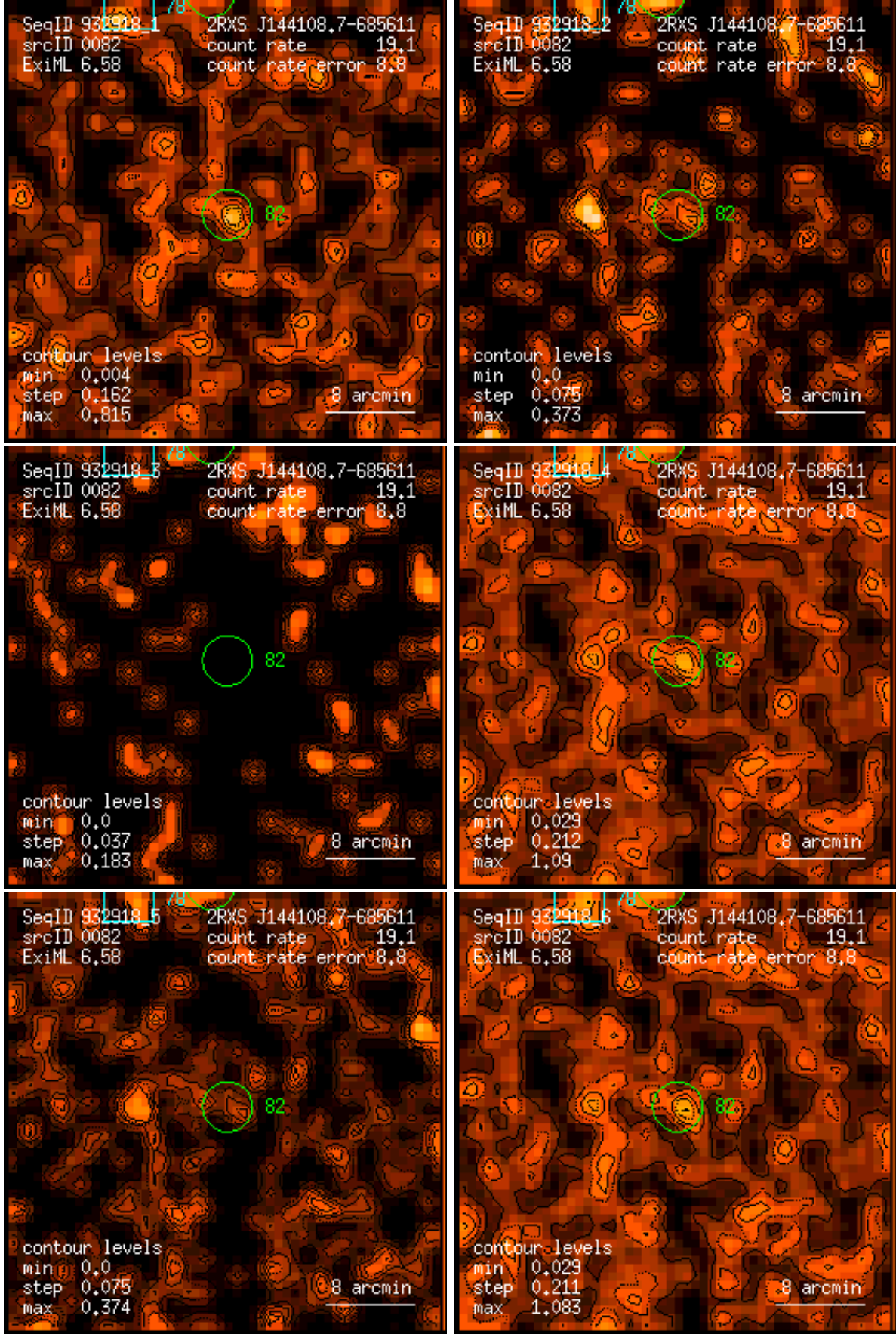
Figure 82: RASS 932918: detection 0082: band rate images, Gaussian filter: (1) PSPC channels 11 – 41, (2) 52 – 90, (3) 91 – 201, (4) 11 – 235, (5) 52 – 201, (6) 11 – 201. Broad band rates in counts/ks. Band rate contour levels in counts/ks/arcmin 2 .
