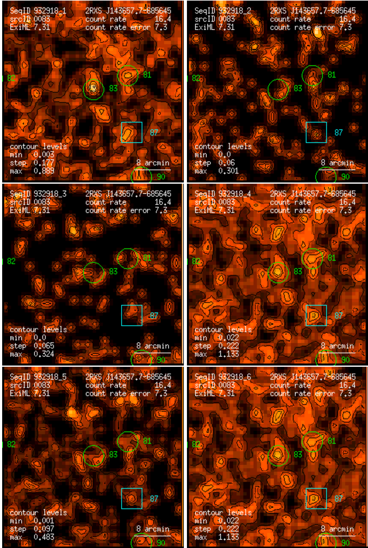
Figure 83: RASS 932918: detection 0083: band rate images, Gaussian filter: (1) PSPC channels 11 – 41, (2) 52 – 90, (3) 91 – 201, (4) 11 – 235, (5) 52 – 201, (6) 11 – 201. Broad band rates in counts/ks. Band rate contour levels in counts/ks/arcmin 2 .
