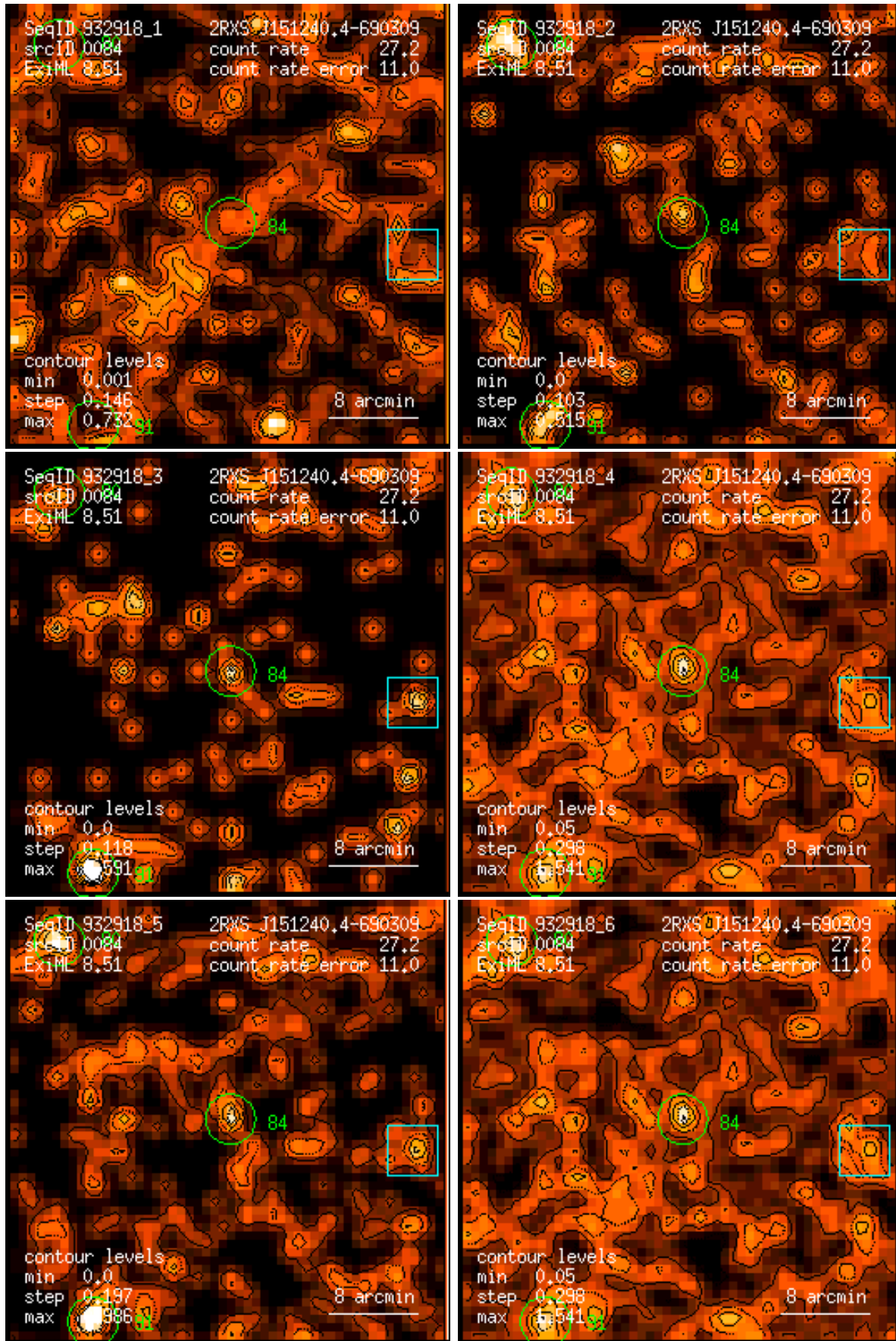
Figure 84: RASS 932918: detection 0084: band rate images, Gaussian filter: (1) PSPC channels 11 – 41, (2) 52 – 90, (3) 91 – 201, (4) 11 – 235, (5) 52 – 201, (6) 11 – 201. Broad band rates in counts/ks. Band rate contour levels in counts/ks/arcmin 2 .
