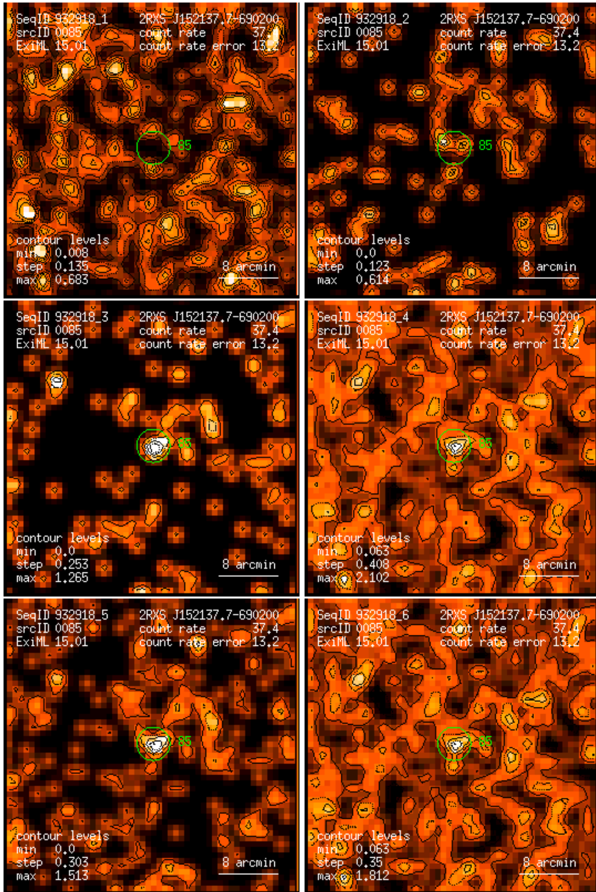
Figure 85: RASS 932918: detection 0085: band rate images, Gaussian filter: (1) PSPC channels 11 – 41, (2) 52 – 90, (3) 91 – 201, (4) 11 – 235, (5) 52 – 201, (6) 11 – 201. Broad band rates in counts/ks. Band rate contour levels in counts/ks/arcmin 2 .
