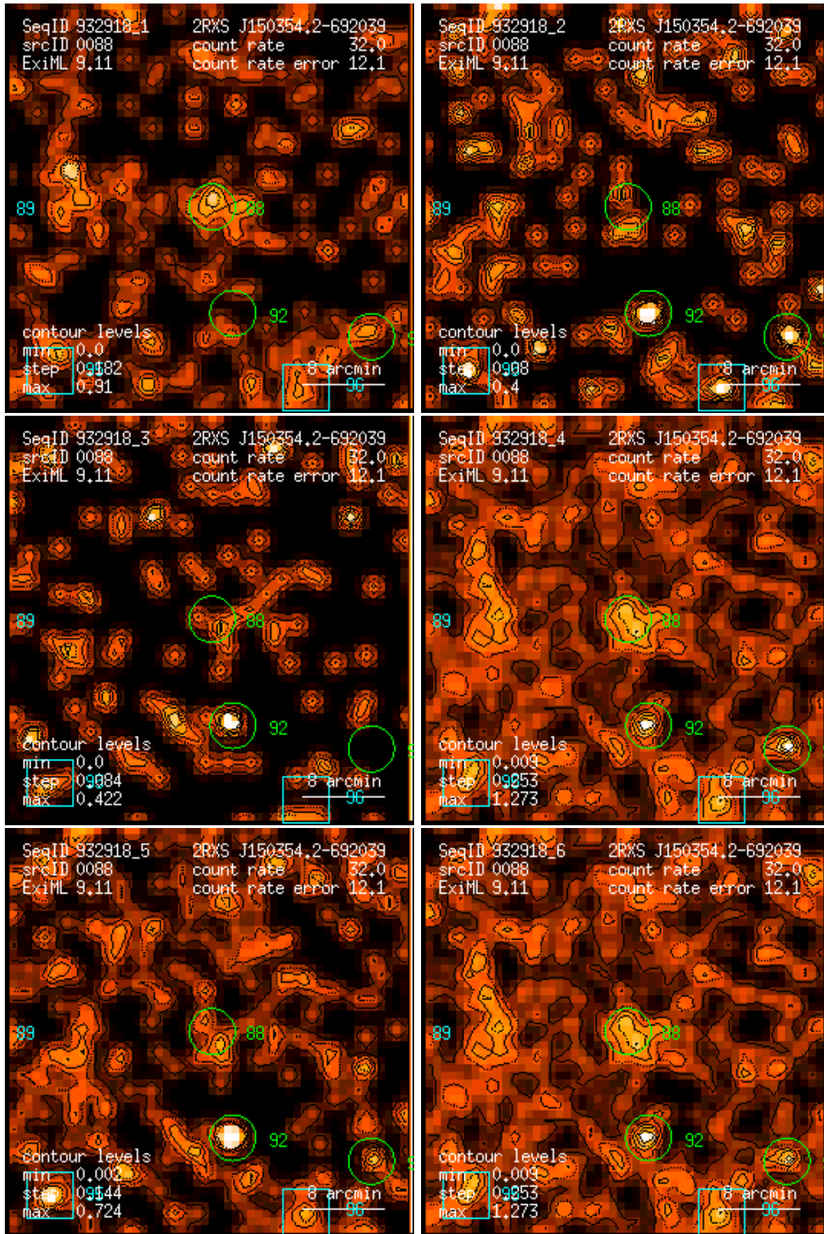
Figure 88: RASS 932918: detection 0088: band rate images, Gaussian filter: (1) PSPC channels 11 – 41, (2) 52 – 90, (3) 91 – 201, (4) 11 – 235, (5) 52 – 201, (6) 11 – 201. Broad band rates in counts/ks. Band rate contour levels in counts/ks/arcmin 2 .
