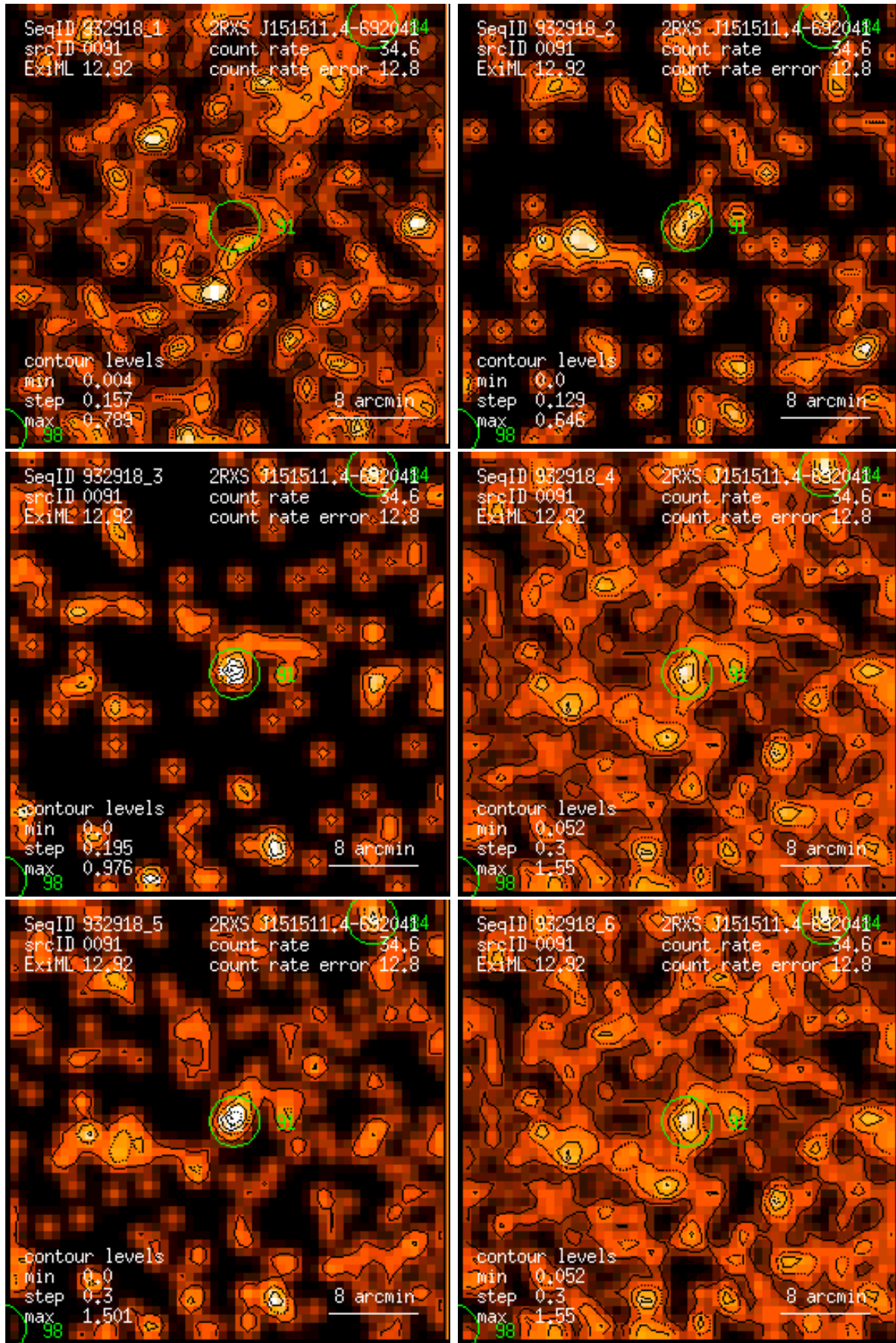
Figure 91: RASS 932918: detection 0091: band rate images, Gaussian filter: (1) PSPC channels 11 – 41, (2) 52 – 90, (3) 91 – 201, (4) 11 – 235, (5) 52 – 201, (6) 11 – 201. Broad band rates in counts/ks. Band rate contour levels in counts/ks/arcmin 2 .
