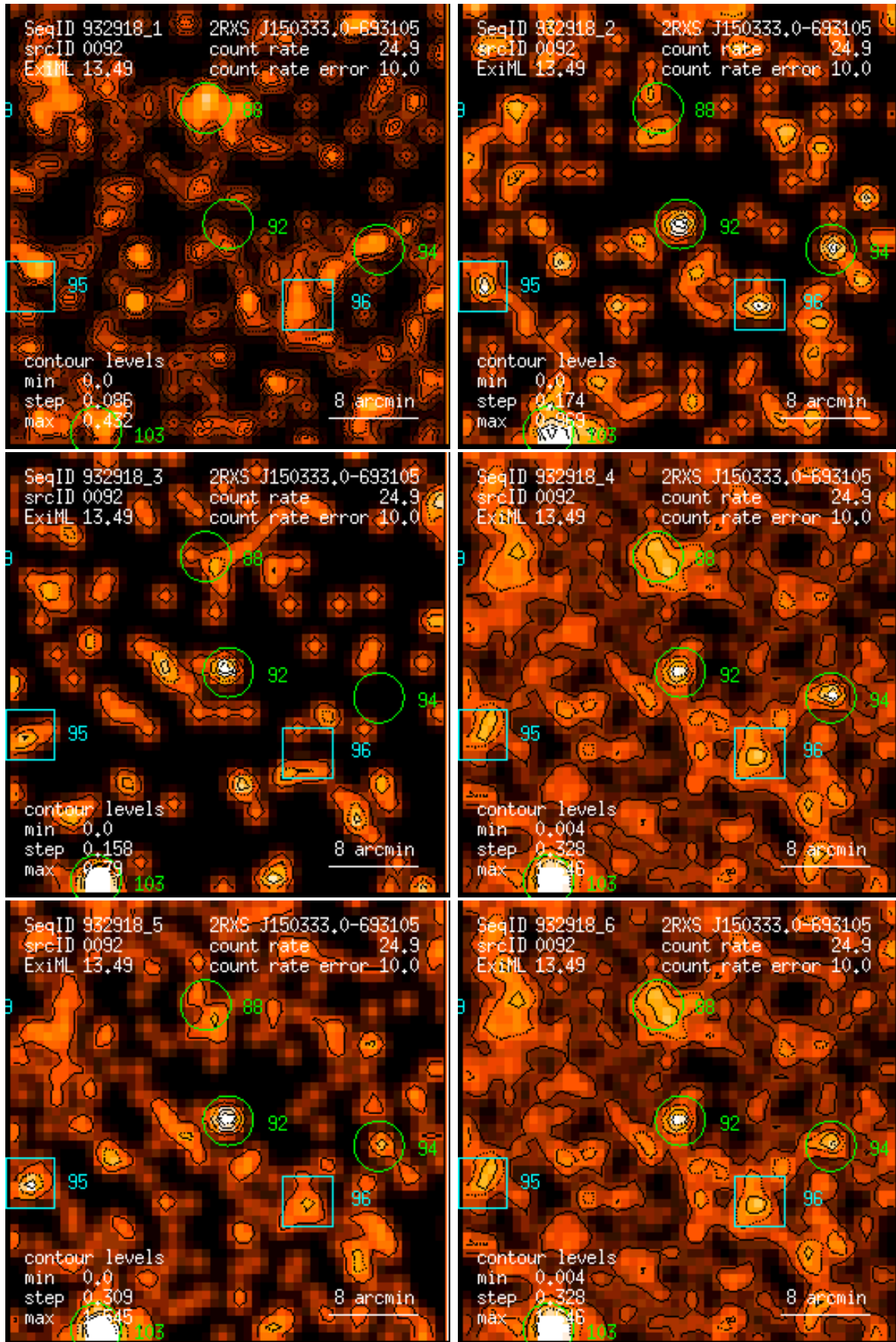
Figure 92: RASS 932918: detection 0092: band rate images, Gaussian filter: (1) PSPC channels 11 – 41, (2) 52 – 90, (3) 91 – 201, (4) 11 – 235, (5) 52 – 201, (6) 11 – 201. Broad band rates in counts/ks. Band rate contour levels in counts/ks/arcmin 2 .
