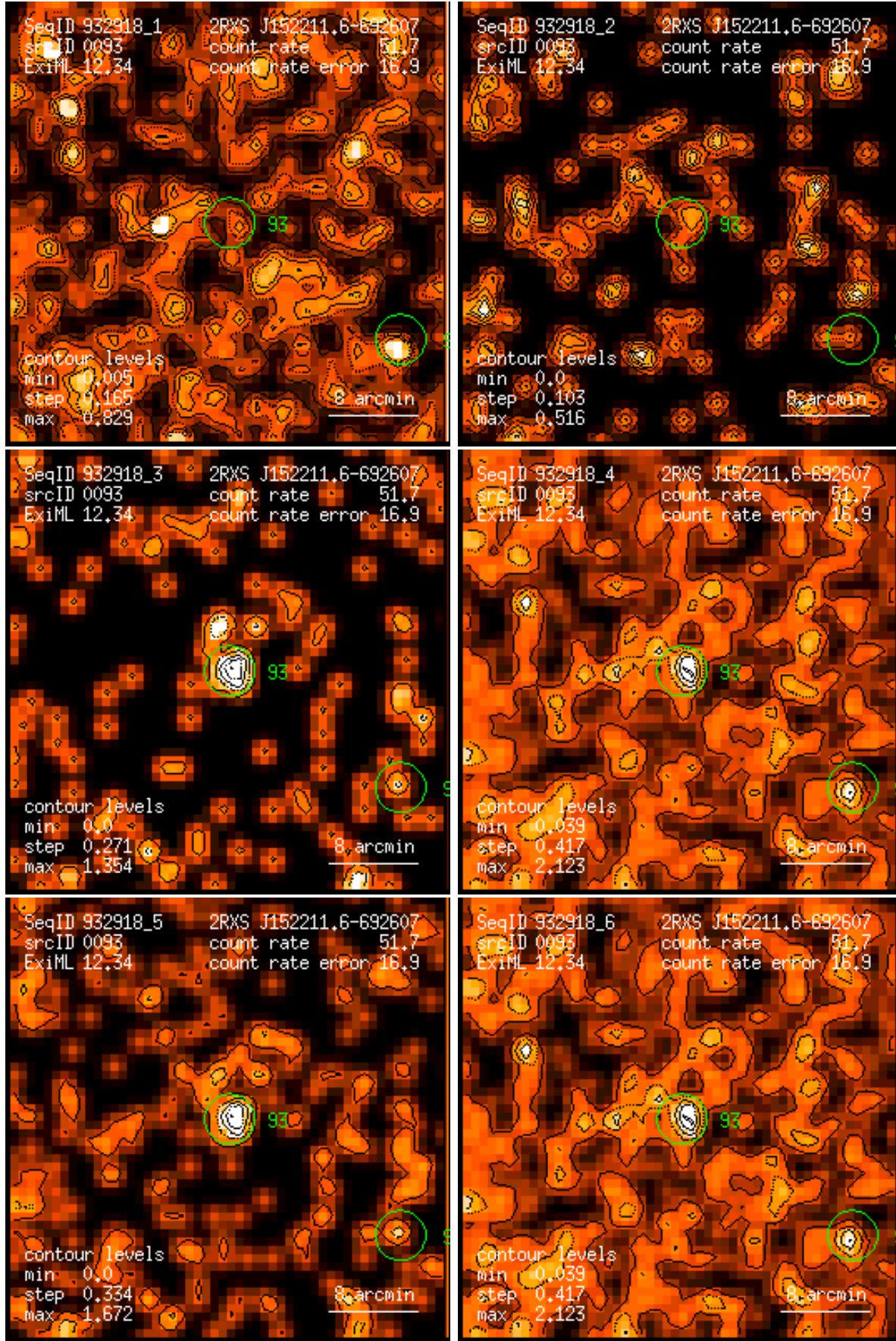
Figure 93: RASS 932918: detection 0093: band rate images, Gaussian filter: (1) PSPC channels 11 – 41, (2) 52 – 90, (3) 91 – 201, (4) 11 – 235, (5) 52 – 201, (6) 11 – 201. Broad band rates in counts/ks. Band rate contour levels in counts/ks/arcmin 2 .
