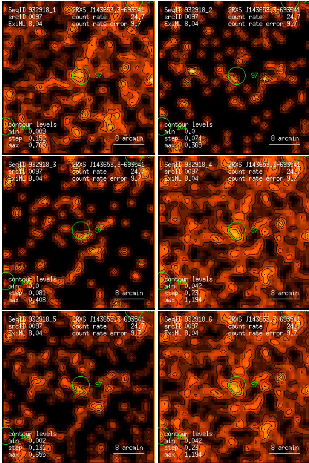
Figure 97: RASS 932918: detection 0097: band rate images, Gaussian filter: (1) PSPC channels 11 – 41, (2) 52 – 90, (3) 91 – 201, (4) 11 – 235, (5) 52 – 201, (6) 11 – 201. Broad band rates in counts/ks. Band rate contour levels in counts/ks/arcmin 2 .
