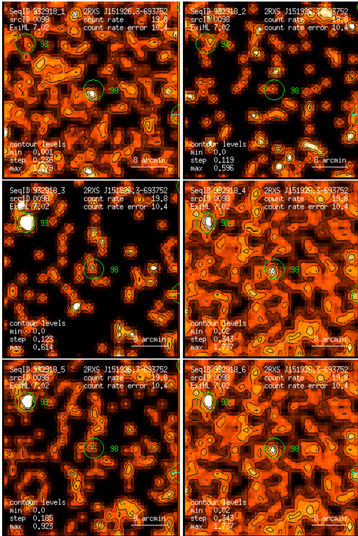
Figure 98: RASS 932918: detection 0098: band rate images, Gaussian filter: (1) PSPC channels 11 – 41, (2) 52 – 90, (3) 91 – 201, (4) 11 – 235, (5) 52 – 201, (6) 11 – 201. Broad band rates in counts/ks. Band rate contour levels in counts/ks/arcmin 2 .
