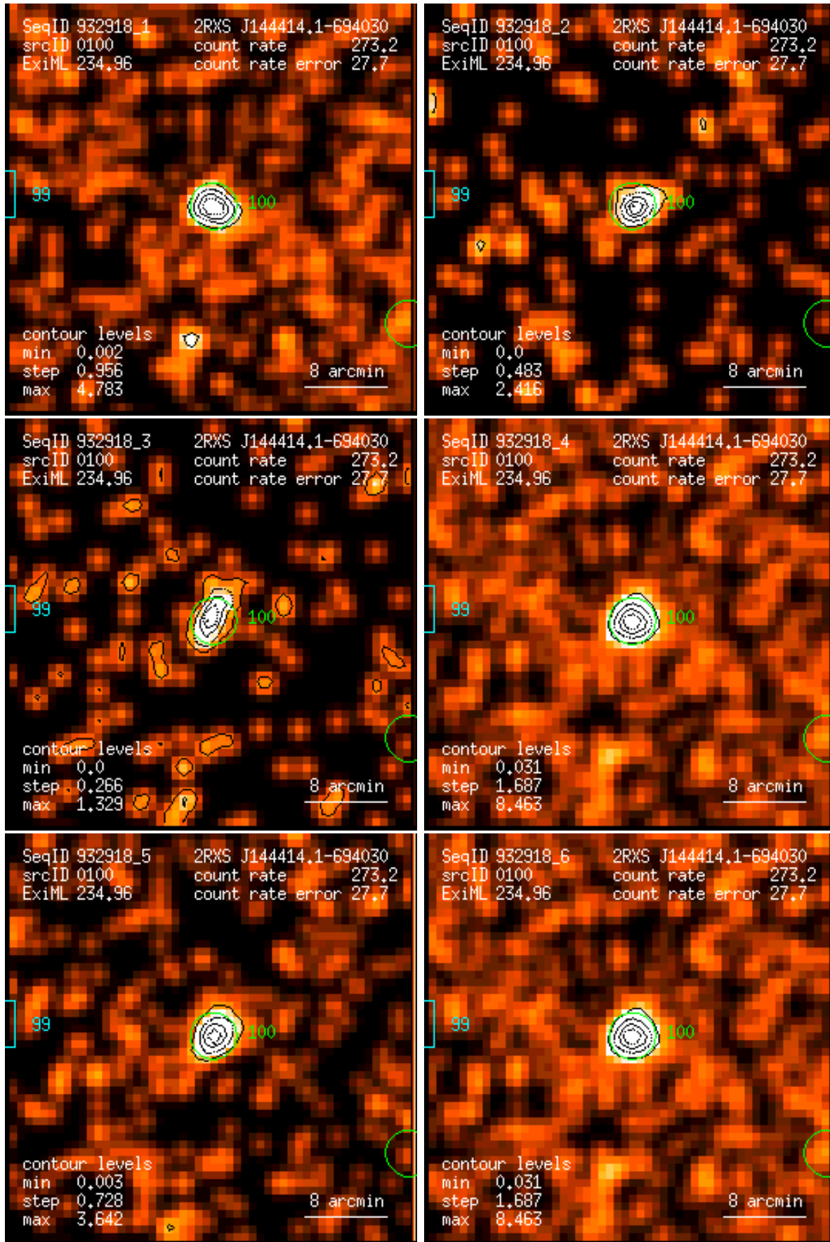
Figure 100: RASS 932918: detection 0100: band rate images, Gaussian filter: (1) PSPC channels 11 – 41, (2) 52 – 90, (3) 91 – 201, (4) 11 – 235, (5) 52 – 201, (6) 11 – 201. Broad band rates in counts/ks. Band rate contour levels in counts/ks/arcmin 2 .
