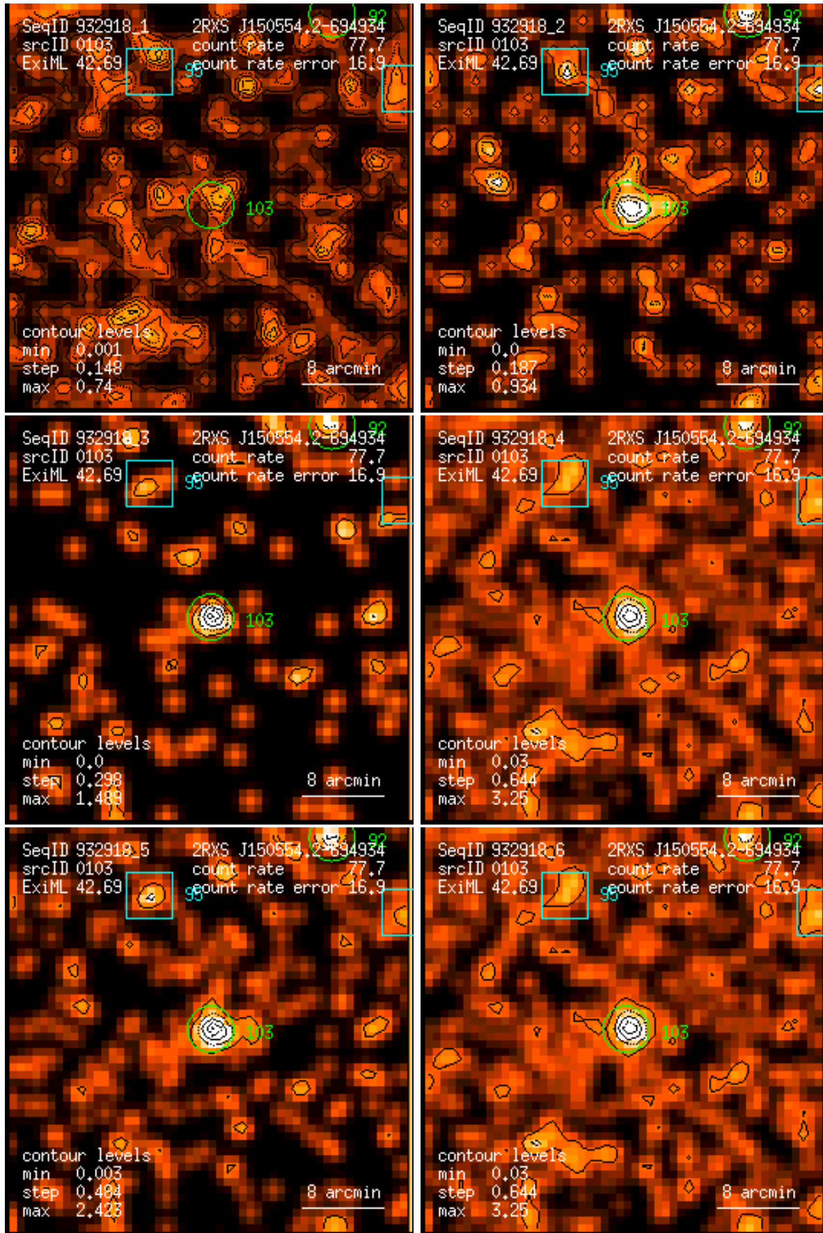
Figure 103: RASS 932918: detection 0103: band rate images, Gaussian filter: (1) PSPC channels 11 – 41, (2) 52 – 90, (3) 91 – 201, (4) 11 – 235, (5) 52 – 201, (6) 11 – 201. Broad band rates in counts/ks. Band rate contour levels in counts/ks/arcmin 2 .
