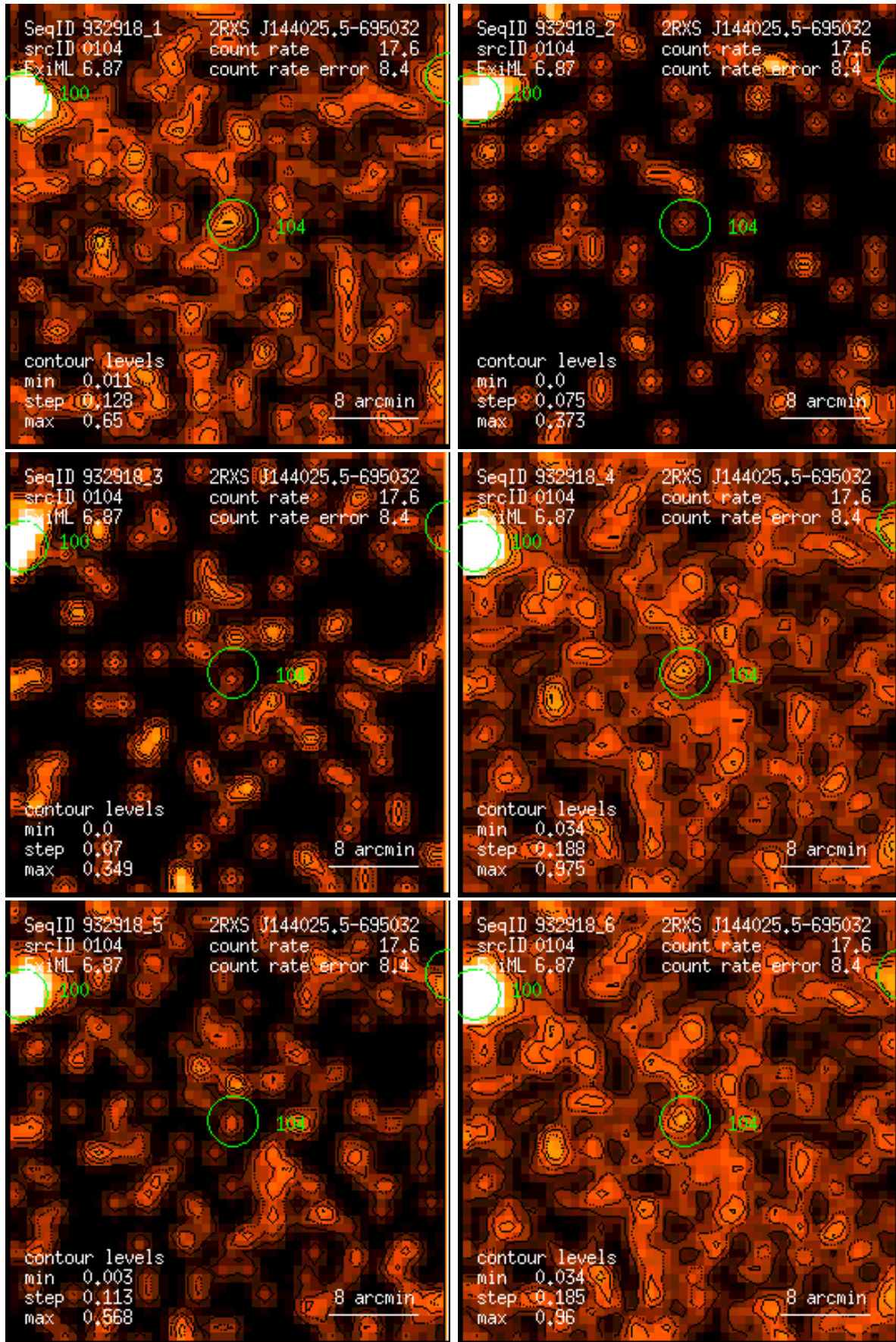
Figure 104: RASS 932918: detection 0104: band rate images, Gaussian filter: (1) PSPC channels 11 – 41, (2) 52 – 90, (3) 91 – 201, (4) 11 – 235, (5) 52 – 201, (6) 11 – 201. Broad band rates in counts/ks. Band rate contour levels in counts/ks/arcmin 2 .
