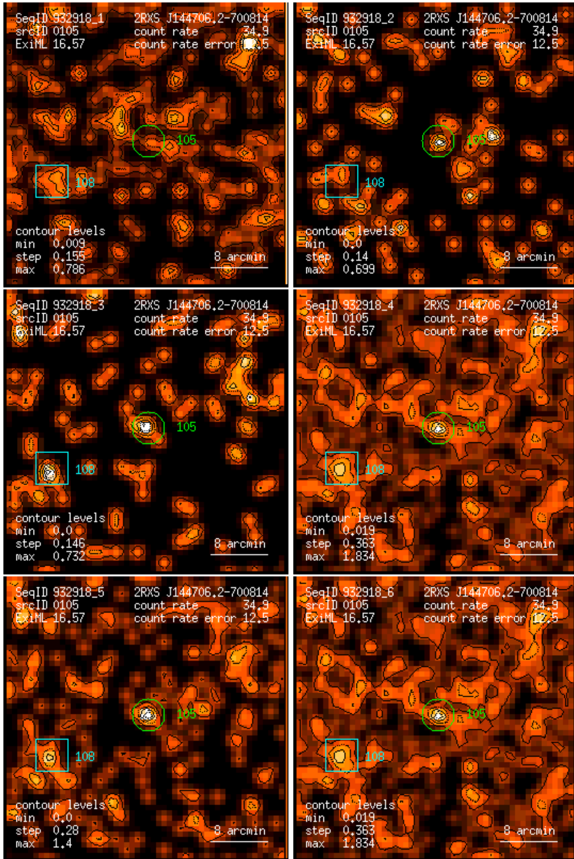
Figure 105: RASS 932918: detection 0105: band rate images, Gaussian filter: (1) PSPC channels 11 – 41, (2) 52 – 90, (3) 91 – 201, (4) 11 – 235, (5) 52 – 201, (6) 11 – 201. Broad band rates in counts/ks. Band rate contour levels in counts/ks/arcmin 2 .
