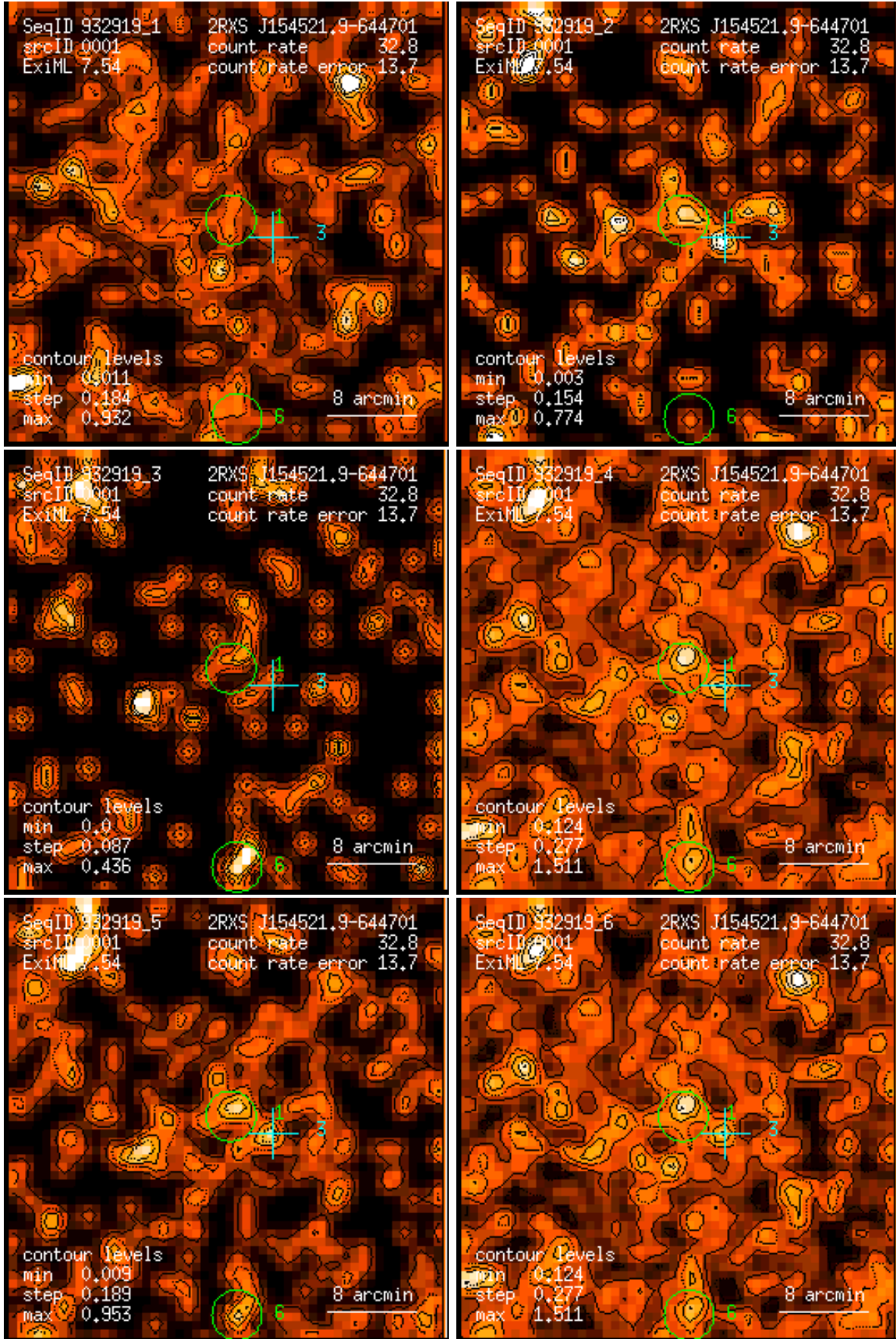
Figure 1: RASS 932919: detection 0001: band rate images, Gaussian filter: (1) PSPC channels 11 – 41, (2) 52 – 90, (3) 91 – 201, (4) 11 – 235, (5) 52 – 201, (6) 11 – 201. Broad band rates in counts/ks. Band rate contour levels in counts/ks/arcmin 2 .
