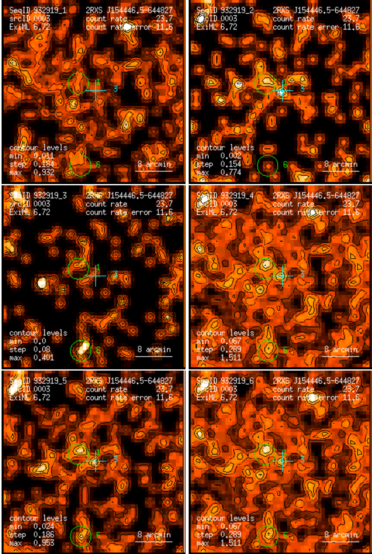
Figure 3: RASS 932919: detection 0003: band rate images, Gaussian filter: (1) PSPC channels 11 – 41, (2) 52 – 90, (3) 91 – 201, (4) 11 – 235, (5) 52 – 201, (6) 11 – 201. Broad band rates in counts/ks. Band rate contour levels in counts/ks/arcmin 2 .
