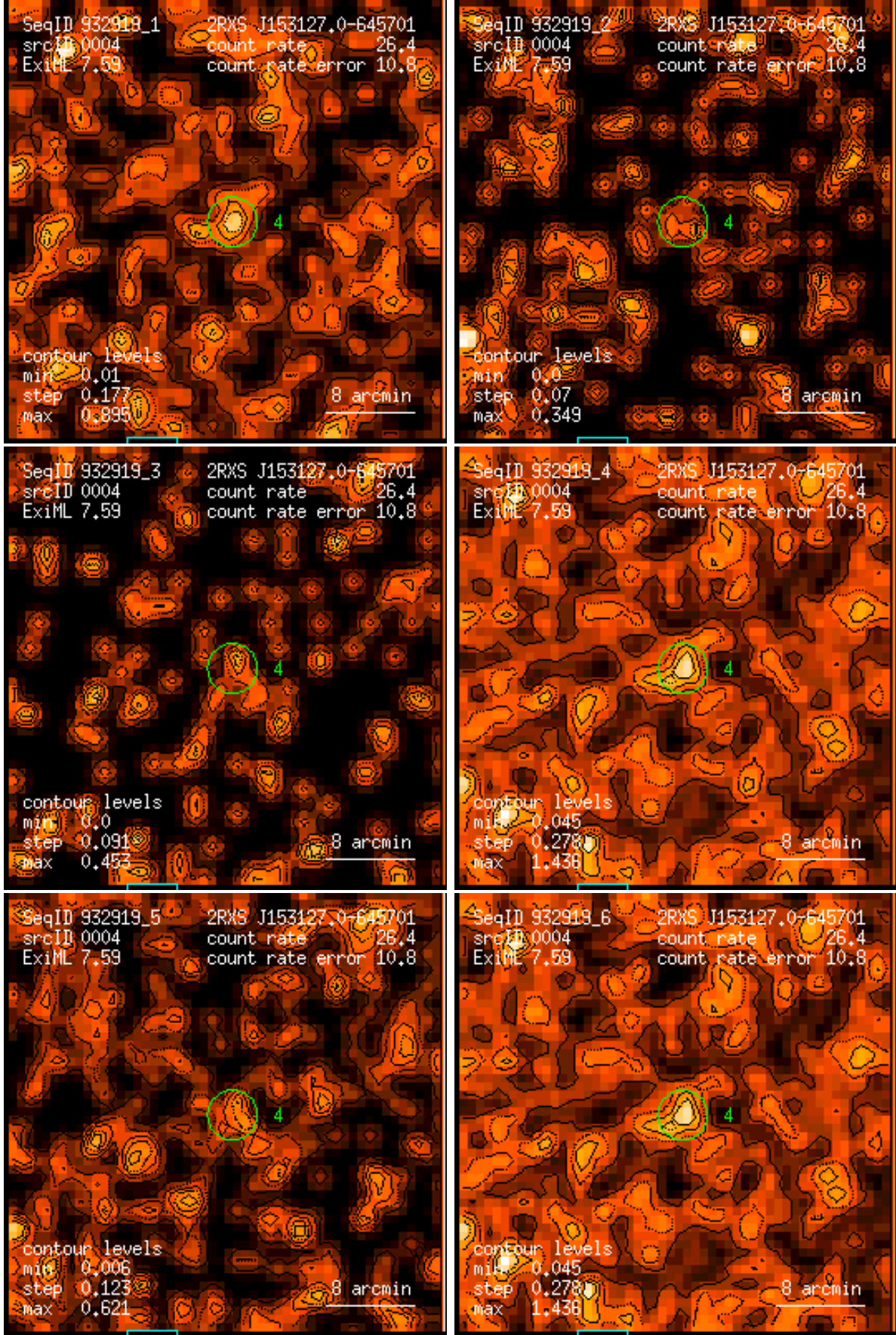
Figure 4: RASS 932919: detection 0004: band rate images, Gaussian filter: (1) PSPC channels 11 – 41, (2) 52 – 90, (3) 91 – 201, (4) 11 – 235, (5) 52 – 201, (6) 11 – 201. Broad band rates in counts/ks. Band rate contour levels in counts/ks/arcmin 2 .
