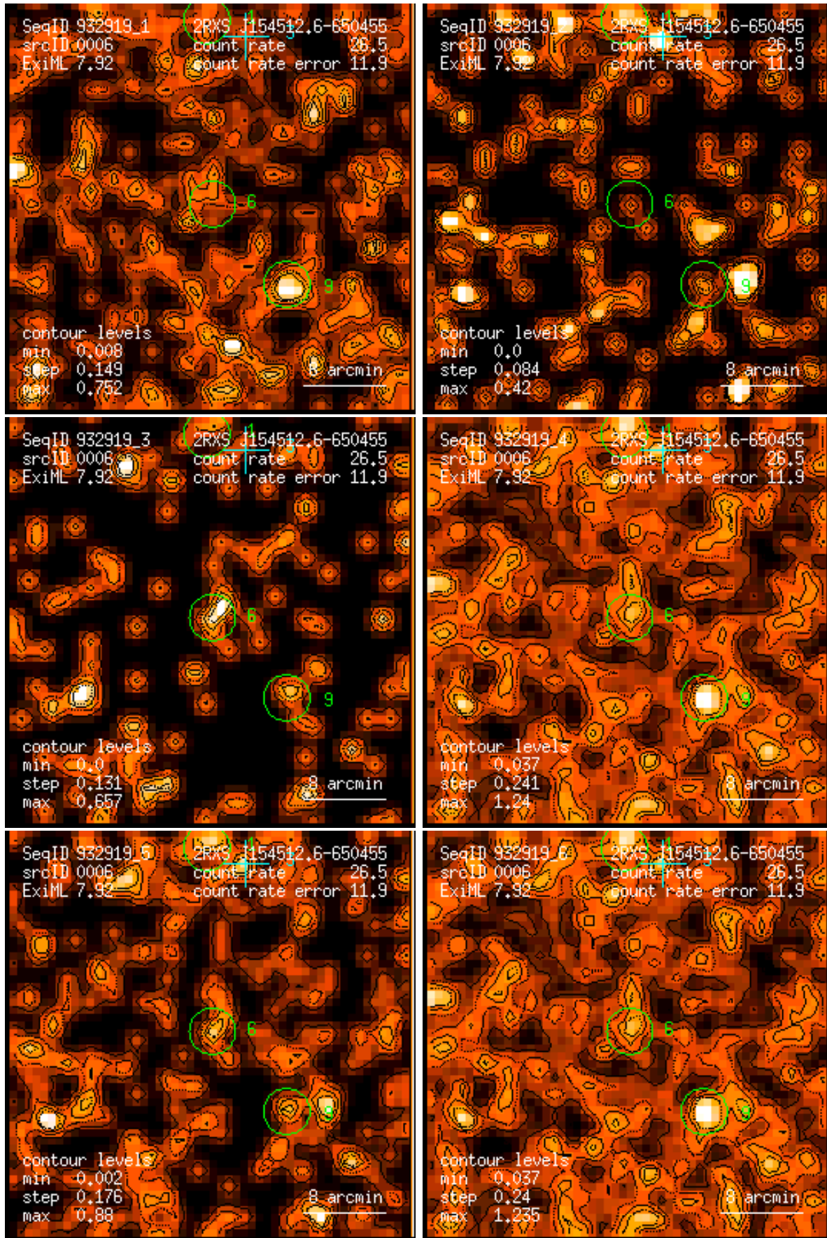
Figure 6: RASS 932919: detection 0006: band rate images, Gaussian filter: (1) PSPC channels 11 – 41, (2) 52 – 90, (3) 91 – 201, (4) 11 – 235, (5) 52 – 201, (6) 11 – 201. Broad band rates in counts/ks. Band rate contour levels in counts/ks/arcmin 2 .
