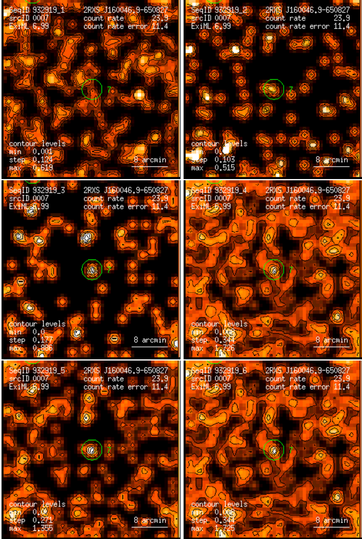
Figure 7: RASS 932919: detection 0007: band rate images, Gaussian filter: (1) PSPC channels 11 – 41, (2) 52 – 90, (3) 91 – 201, (4) 11 – 235, (5) 52 – 201, (6) 11 – 201. Broad band rates in counts/ks. Band rate contour levels in counts/ks/arcmin 2 .
