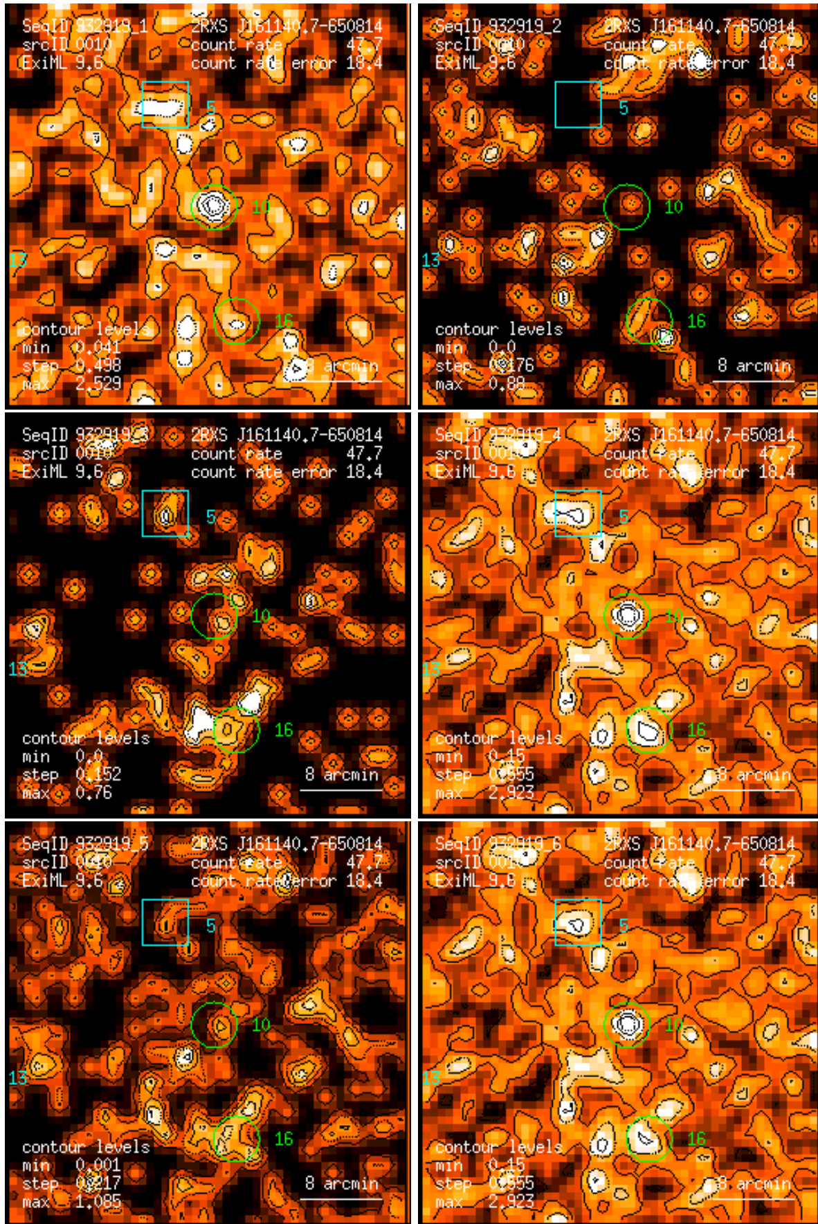
Figure 10: RASS 932919: detection 0010: band rate images, Gaussian filter: (1) PSPC channels 11 – 41, (2) 52 – 90, (3) 91 – 201, (4) 11 – 235, (5) 52 – 201, (6) 11 – 201. Broad band rates in counts/ks. Band rate contour levels in counts/ks/arcmin 2 .
