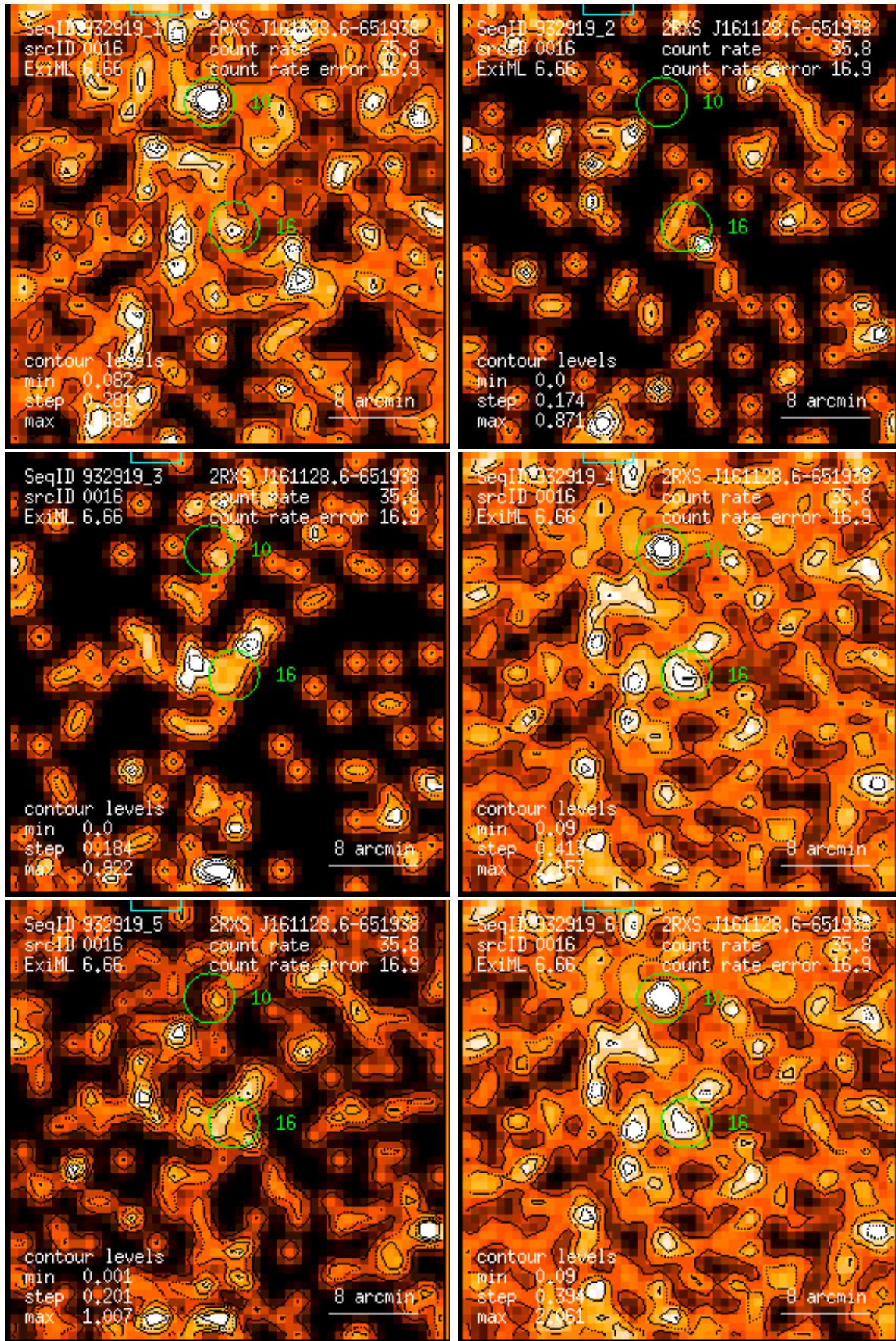
Figure 16: RASS 932919: detection 0016: band rate images, Gaussian filter: (1) PSPC channels 11 – 41, (2) 52 – 90, (3) 91 – 201, (4) 11 – 235, (5) 52 – 201, (6) 11 – 201. Broad band rates in counts/ks. Band rate contour levels in counts/ks/arcmin 2 .
