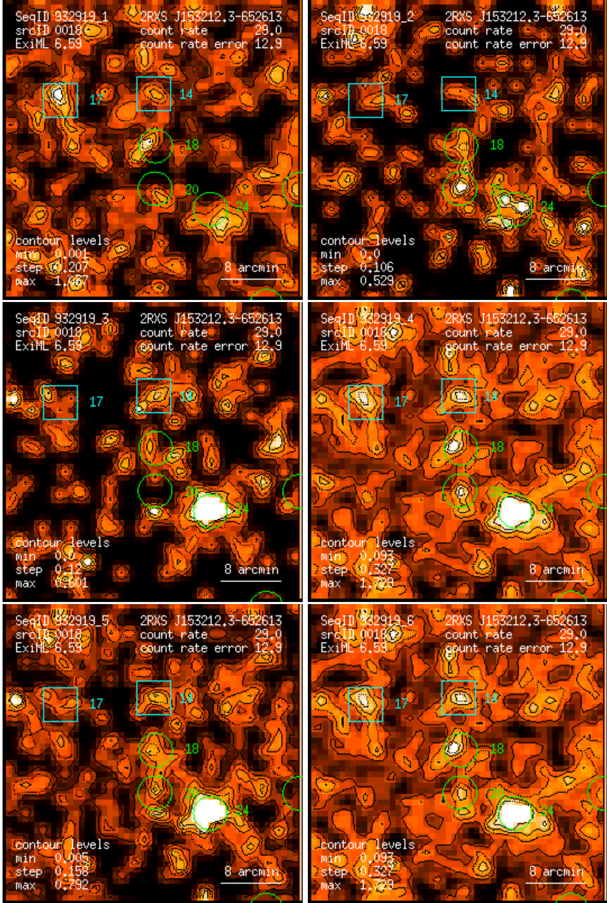
Figure 18: RASS 932919: detection 0018: band rate images, Gaussian filter: (1) PSPC channels 11 – 41, (2) 52 – 90, (3) 91 – 201, (4) 11 – 235, (5) 52 – 201, (6) 11 – 201. Broad band rates in counts/ks. Band rate contour levels in counts/ks/arcmin 2 .
