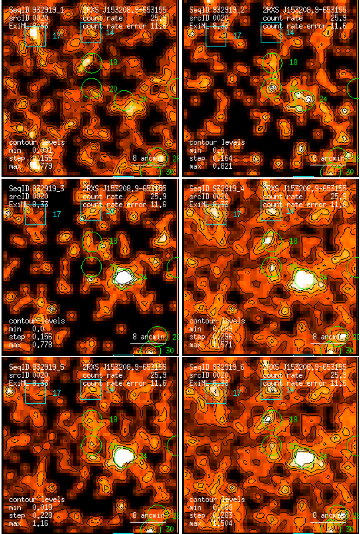
Figure 20: RASS 932919: detection 0020: band rate images, Gaussian filter: (1) PSPC channels 11 – 41, (2) 52 – 90, (3) 91 – 201, (4) 11 – 235, (5) 52 – 201, (6) 11 – 201. Broad band rates in counts/ks. Band rate contour levels in counts/ks/arcmin 2 .
