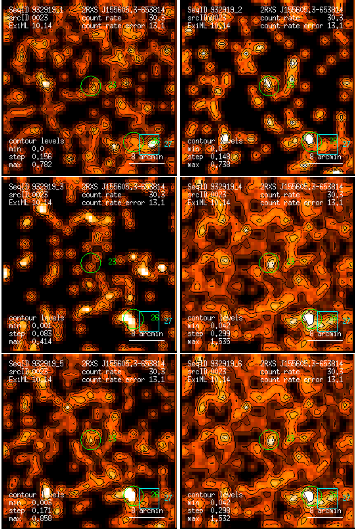
Figure 23: RASS 932919: detection 0023: band rate images, Gaussian filter: (1) PSPC channels 11 – 41, (2) 52 – 90, (3) 91 – 201, (4) 11 – 235, (5) 52 – 201, (6) 11 – 201. Broad band rates in counts/ks. Band rate contour levels in counts/ks/arcmin 2 .
