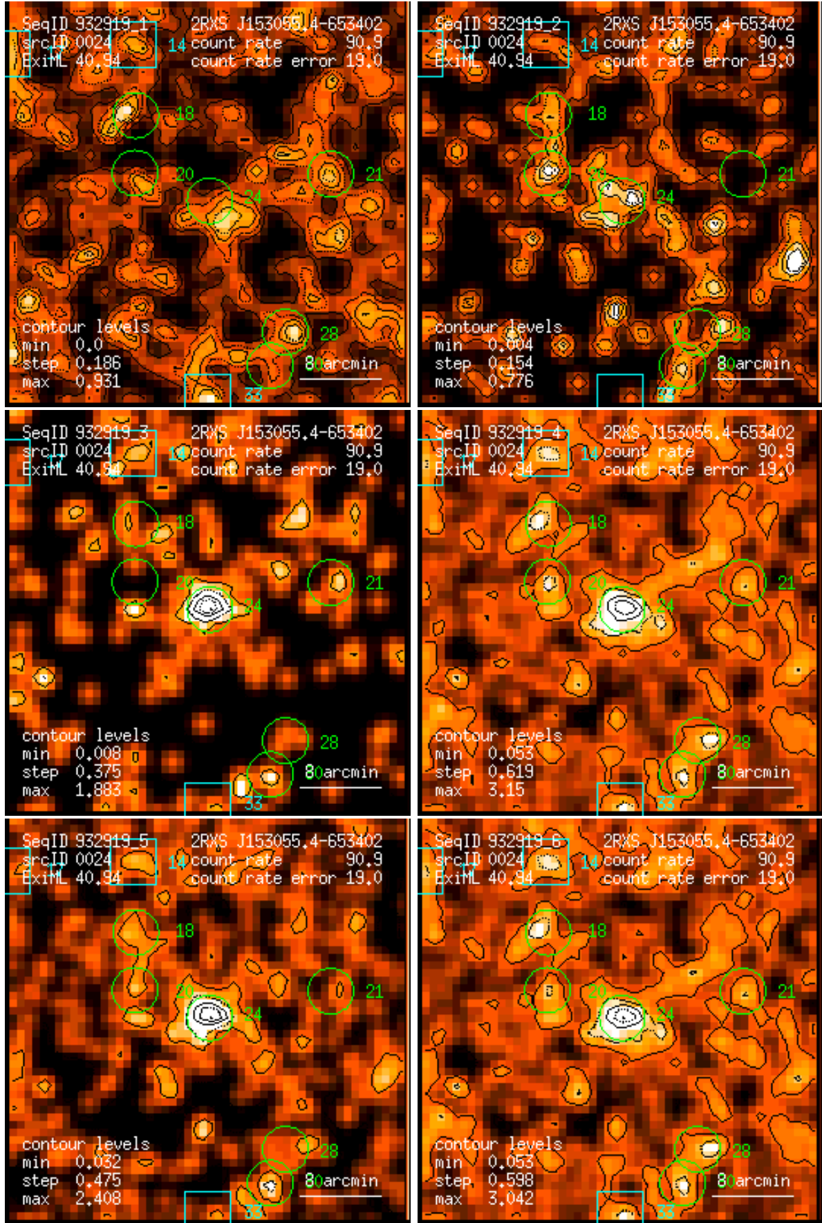
Figure 24: RASS 932919: detection 0024: band rate images, Gaussian filter: (1) PSPC channels 11 – 41, (2) 52 – 90, (3) 91 – 201, (4) 11 – 235, (5) 52 – 201, (6) 11 – 201. Broad band rates in counts/ks. Band rate contour levels in counts/ks/arcmin 2 .
