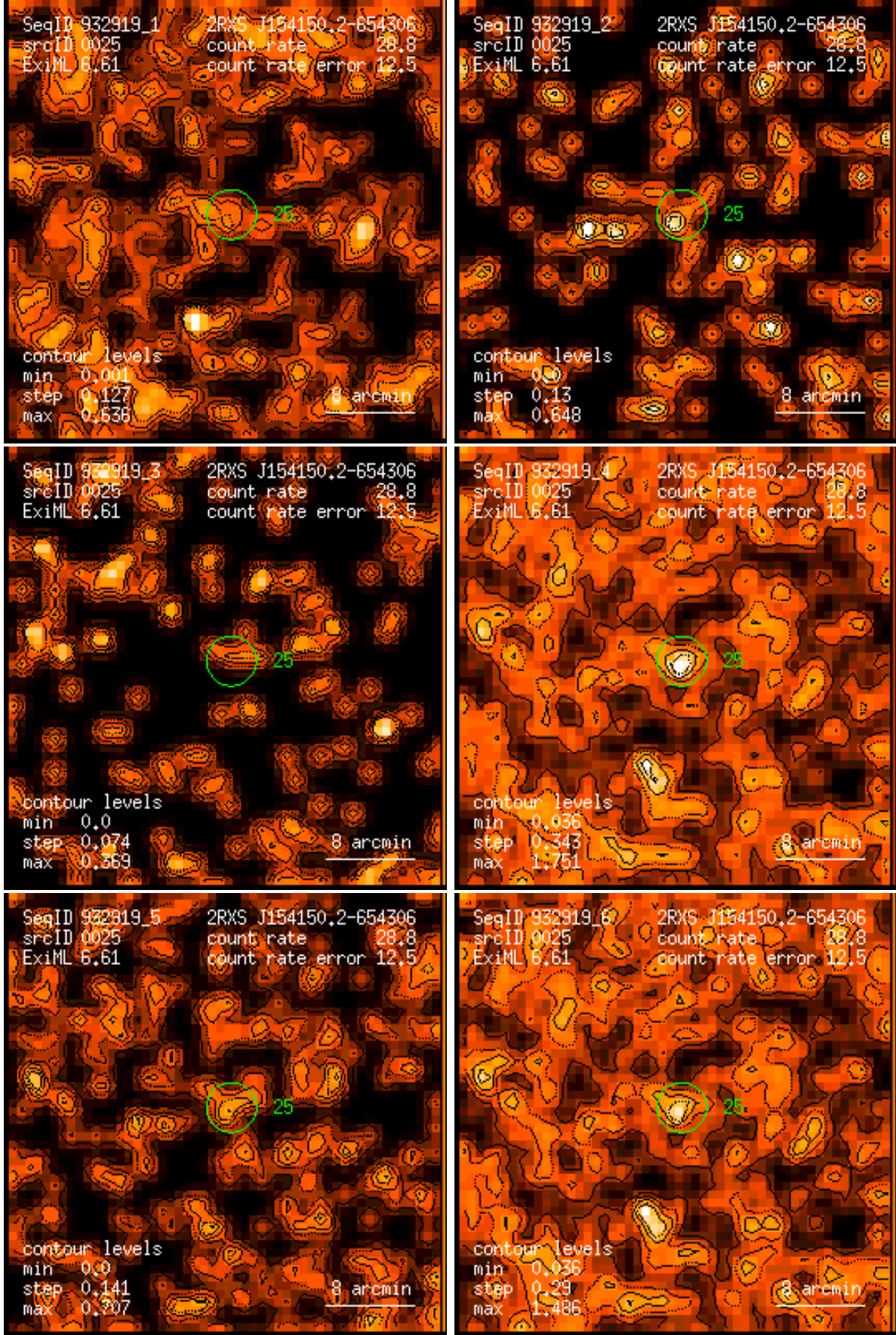
Figure 25: RASS 932919: detection 0025: band rate images, Gaussian filter: (1) PSPC channels 11 – 41, (2) 52 – 90, (3) 91 – 201, (4) 11 – 235, (5) 52 – 201, (6) 11 – 201. Broad band rates in counts/ks. Band rate contour levels in counts/ks/arcmin 2 .
