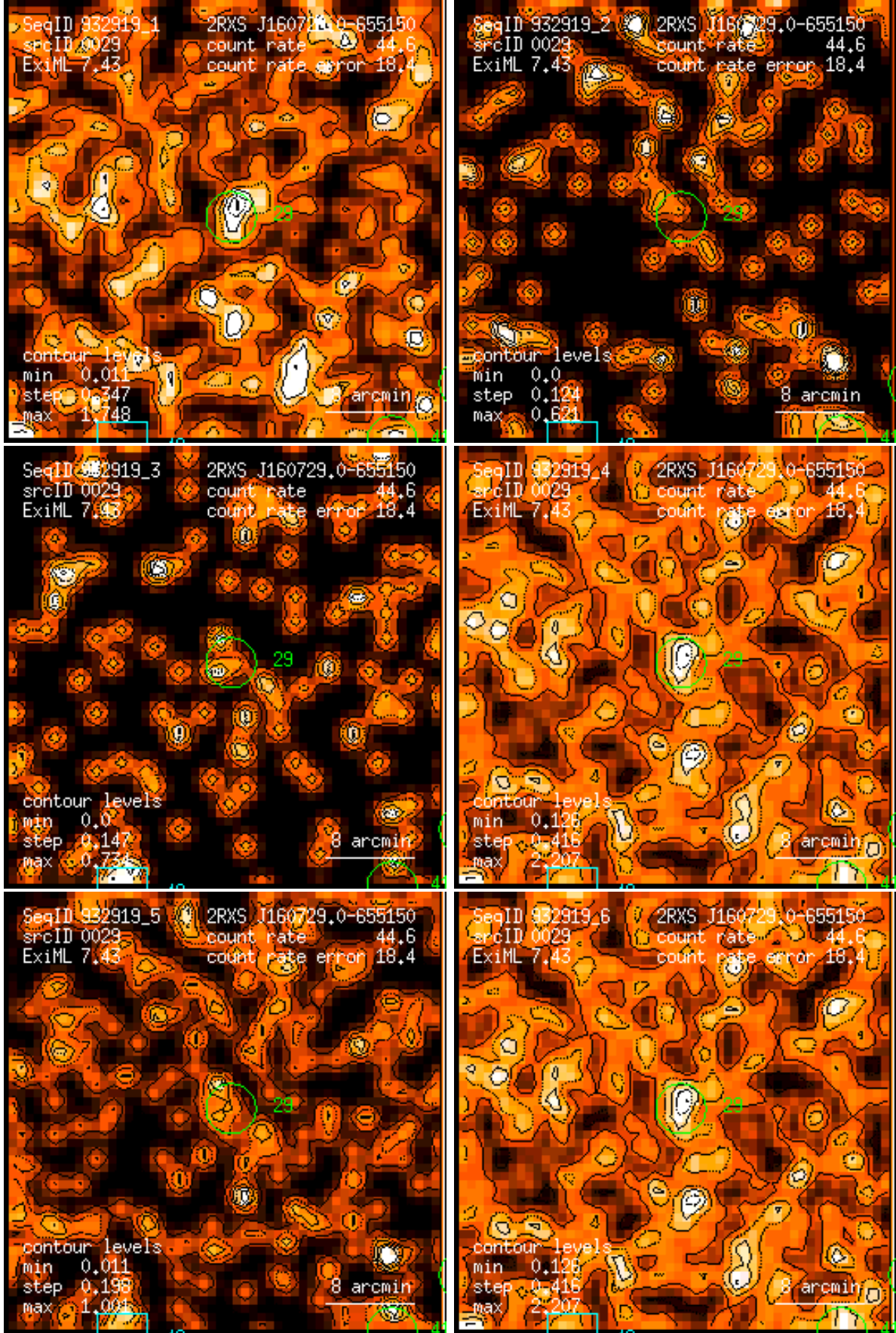
Figure 29: RASS 932919: detection 0029: band rate images, Gaussian filter: (1) PSPC channels 11 – 41, (2) 52 – 90, (3) 91 – 201, (4) 11 – 235, (5) 52 – 201, (6) 11 – 201. Broad band rates in counts/ks. Band rate contour levels in counts/ks/arcmin 2 .
